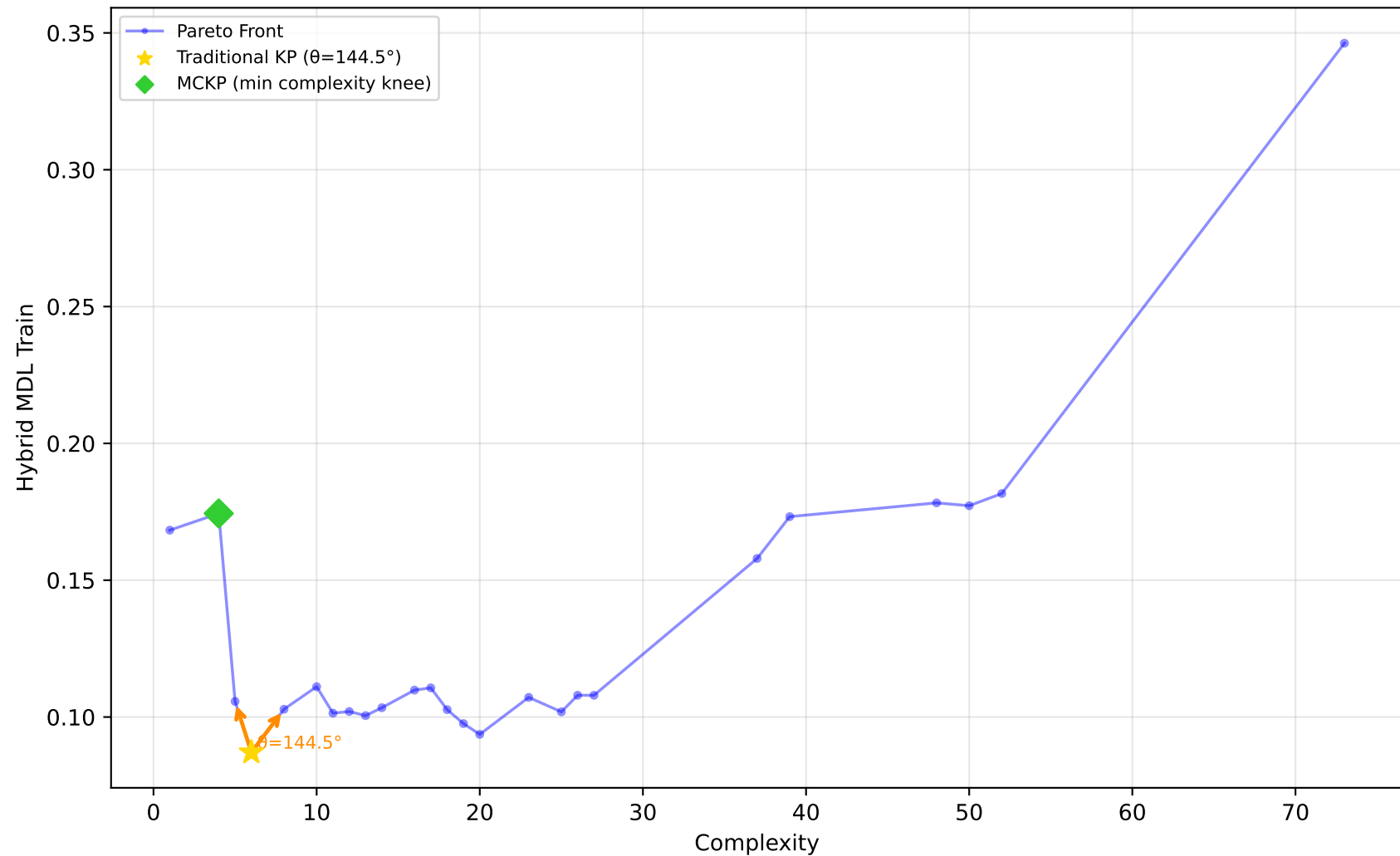
1028_SWD - Run 29 - SVP - Hybrid MDL Train \lambda_1=0.60, \lambda_2=0.00, \lambda_3=0.00 | Difficulty: 1.00 | Method: hmr
