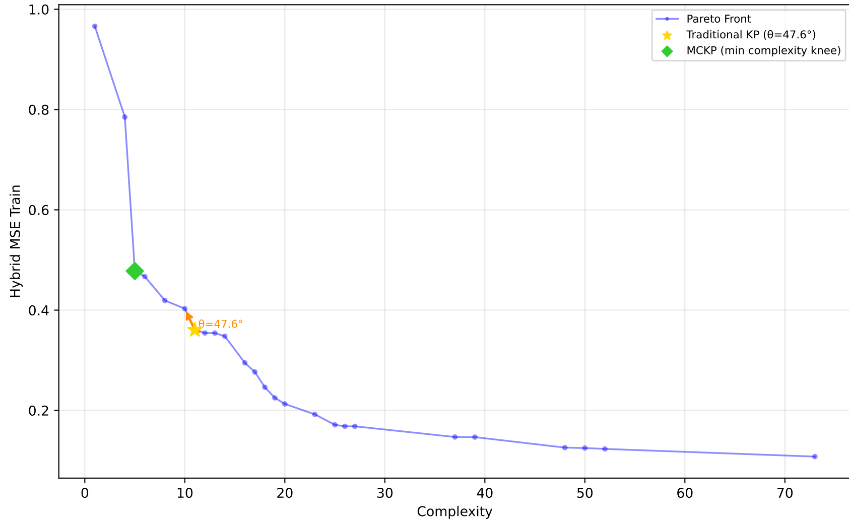
1028_SWD - Run 29 - SVP - Hybrid MSE Train \lambda_1=0.00, \lambda_2=0.60, \lambda_3=0.00 | Difficulty: 1.00 | Method: hmr
