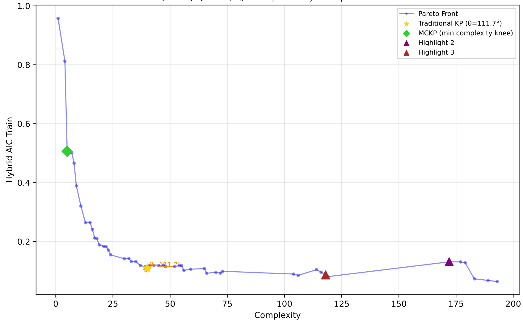
1028_SW_D - Run 2 - MVP - Hybrid AIC Train \lambda_1=0.00, \lambda_2=0.00, \lambda_3=0.00 | Difficulty: 1.00 | Method: hmr
