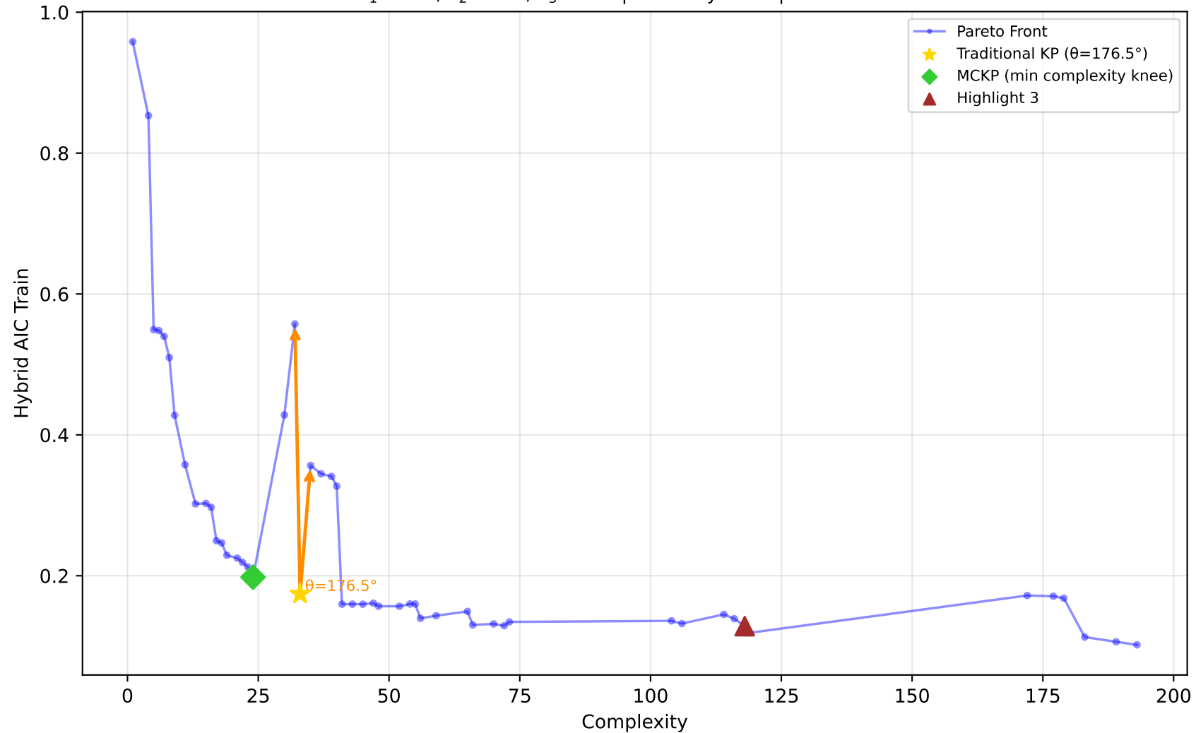
1028_SW_D - Run 2 - MVP - Hybrid AIC Train \lambda_1=0.60, \lambda_2=0.00, \lambda_3=0.00 | Difficulty: 1.00 | Method: hmr
