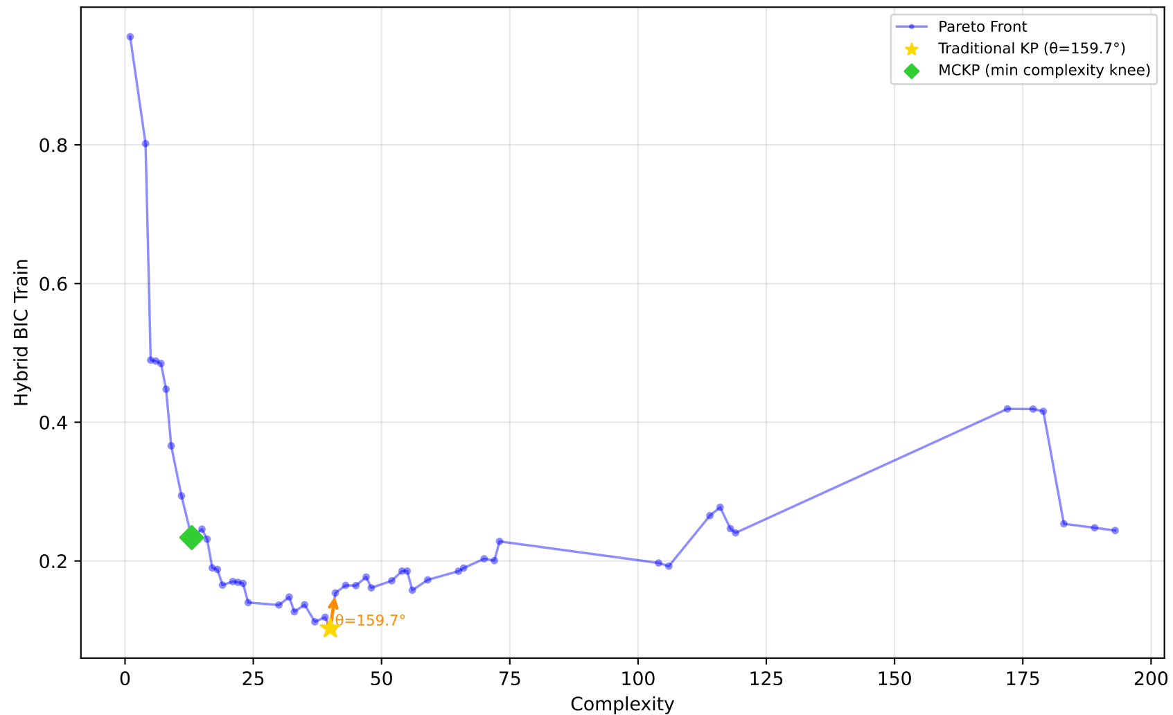
1028_SW_D - Run 2 - MVP - Hybrid BIC Train \lambda_1=0.00, \lambda_2=0.00, \lambda_3=0.00 | Difficulty: 1.00 | Method: hmr
