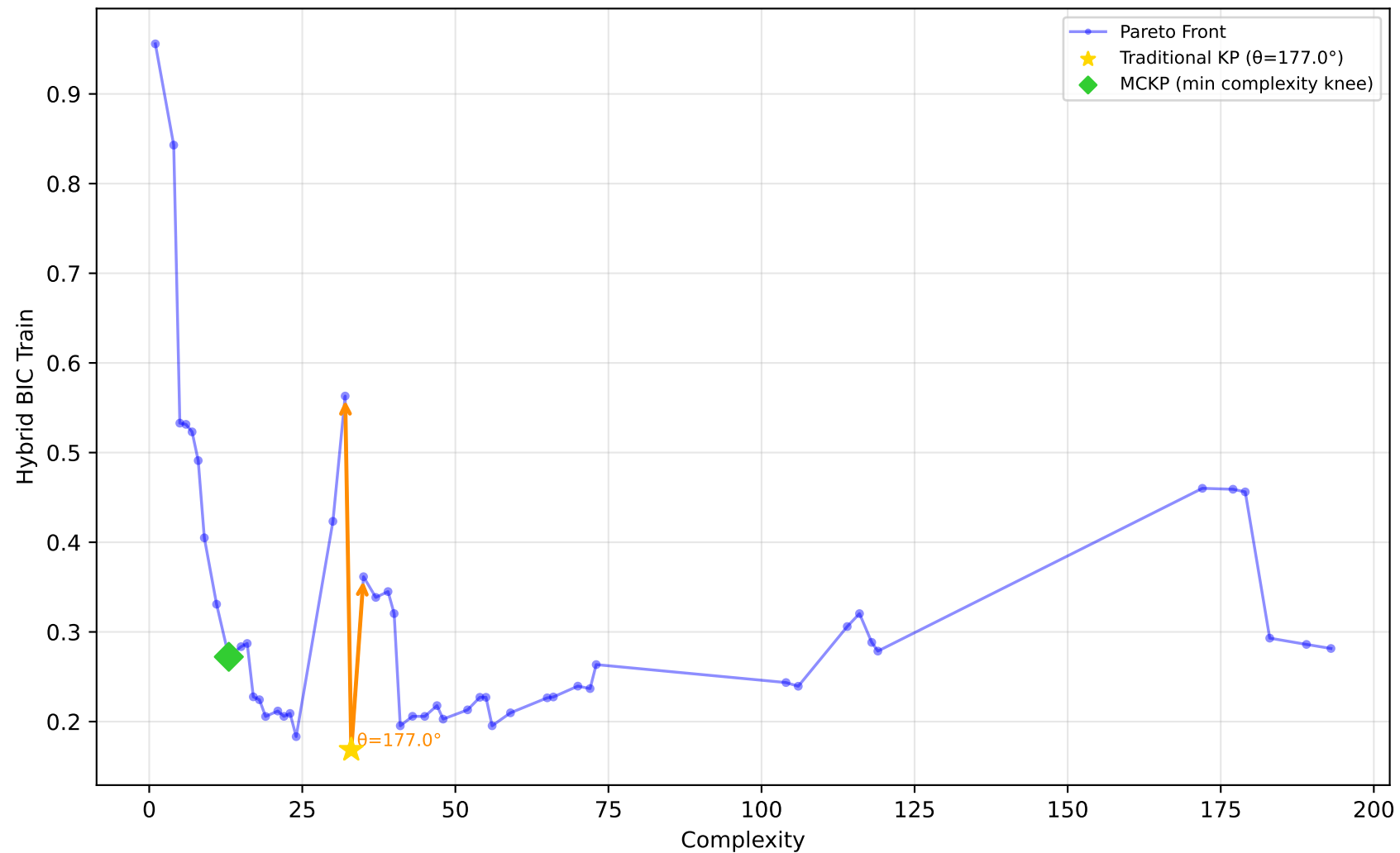
1028_SWD - Run 2 - MVP - Hybrid BIC Train \lambda_1=0.60, \lambda_2=0.00, \lambda_3=0.00 | Difficulty: 1.00 | Method: hmr
