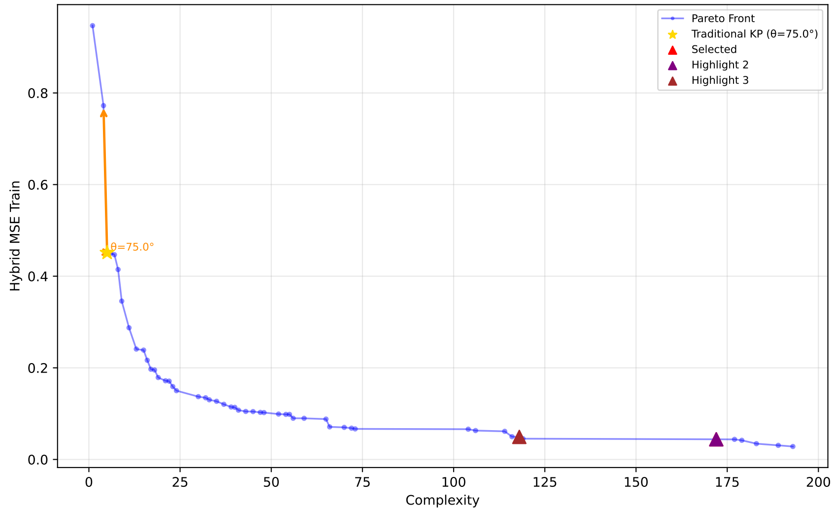
1028_SWD - Run 2 - MVP - Hybrid MSE Train \lambda_1=0.00, \lambda_2=0.00, \lambda_3=0.00 | Difficulty: 1.00 | Method: hmr
