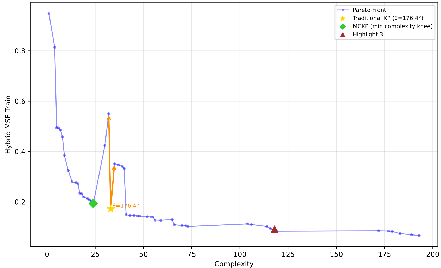
1028_SWD - Run 2 - MVP - Hybrid MSE Train \lambda_1=0.60, \lambda_2=0.00, \lambda_3=0.00 | Difficulty: 1.00 | Method: hmr
