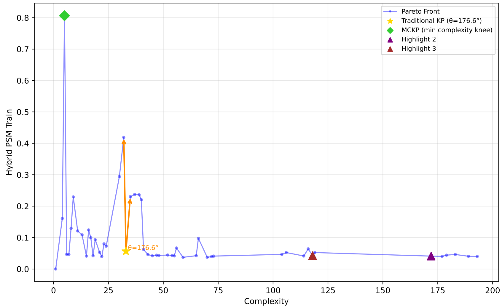
1028_SW_D - Run 2 - MVP - Hybrid PSM Train \lambda_1=0.60, \lambda_2=0.00, \lambda_3=0.00 | Difficulty: 1.00 | Method: hmr
