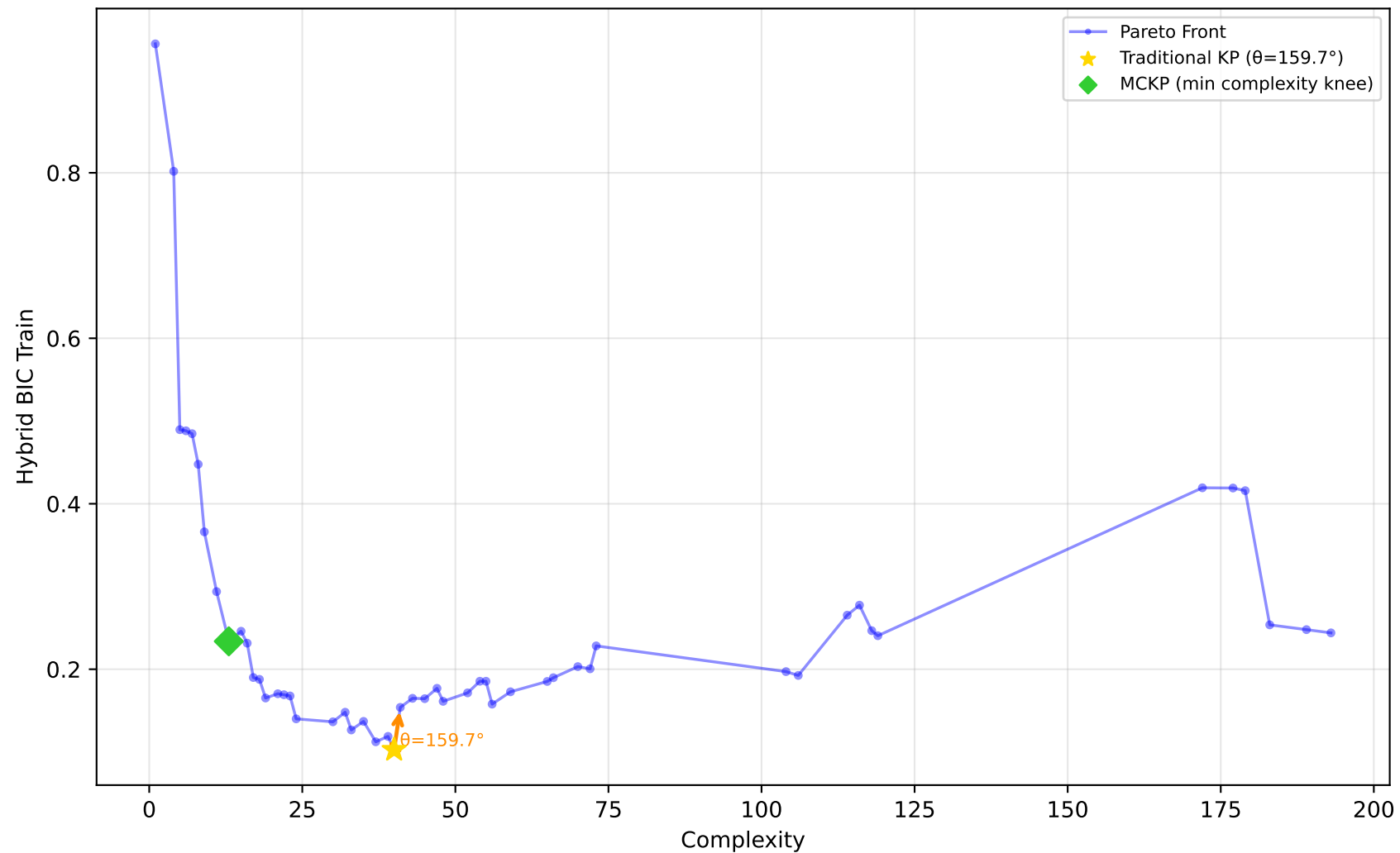
1028_SWD - Run 2 - SVP - Hybrid BIC Train \lambda_1=0.00, \lambda_2=0.60, \lambda_3=0.00 | Difficulty: 1.00 | Method: hmr
