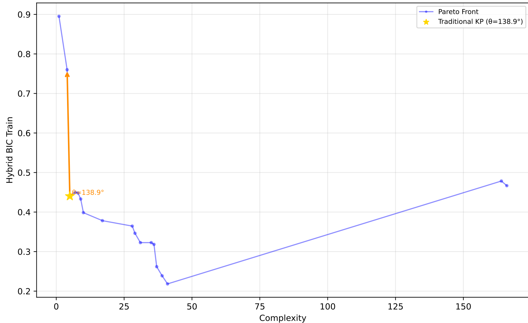
1028_SWD - Run 30 - MVP - Hybrid BIC Train \lambda_1=0.00, \lambda_2=0.00, \lambda_3=0.00 | Difficulty: 1.00 | Method: hmr
