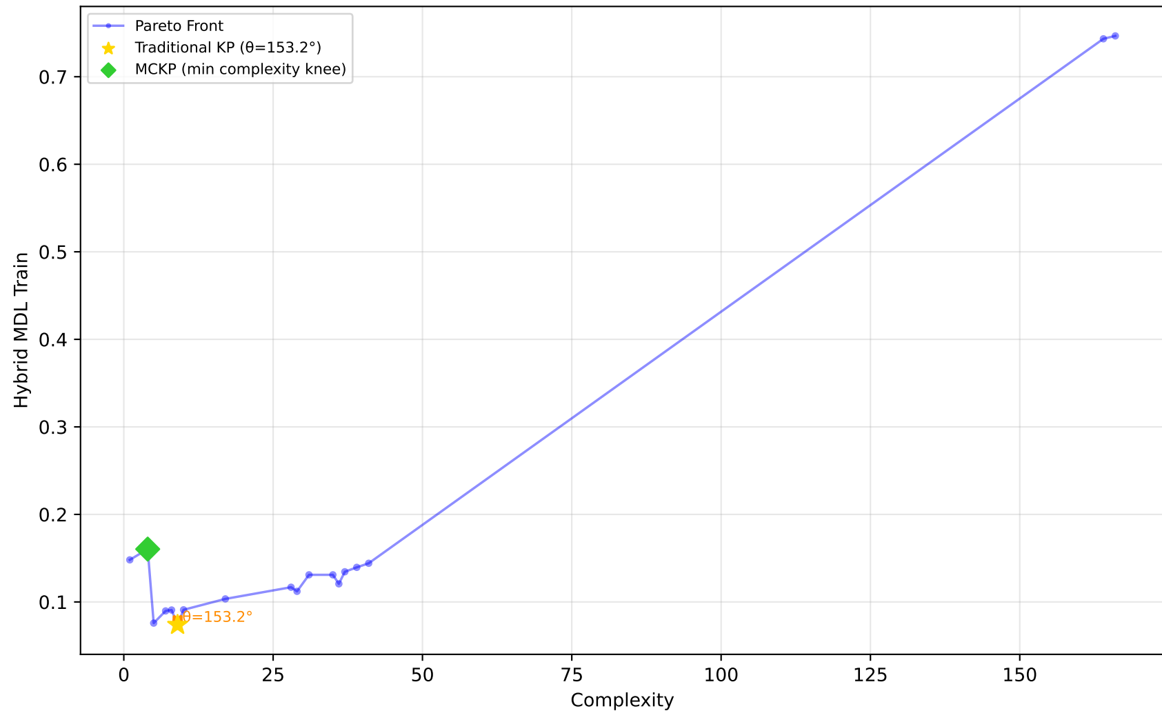
1028_SWD - Run 30 - MVP - Hybrid MDL Train \lambda_1=0.60, \lambda_2=0.00, \lambda_3=0.00 | Difficulty: 1.00 | Method: hmr
