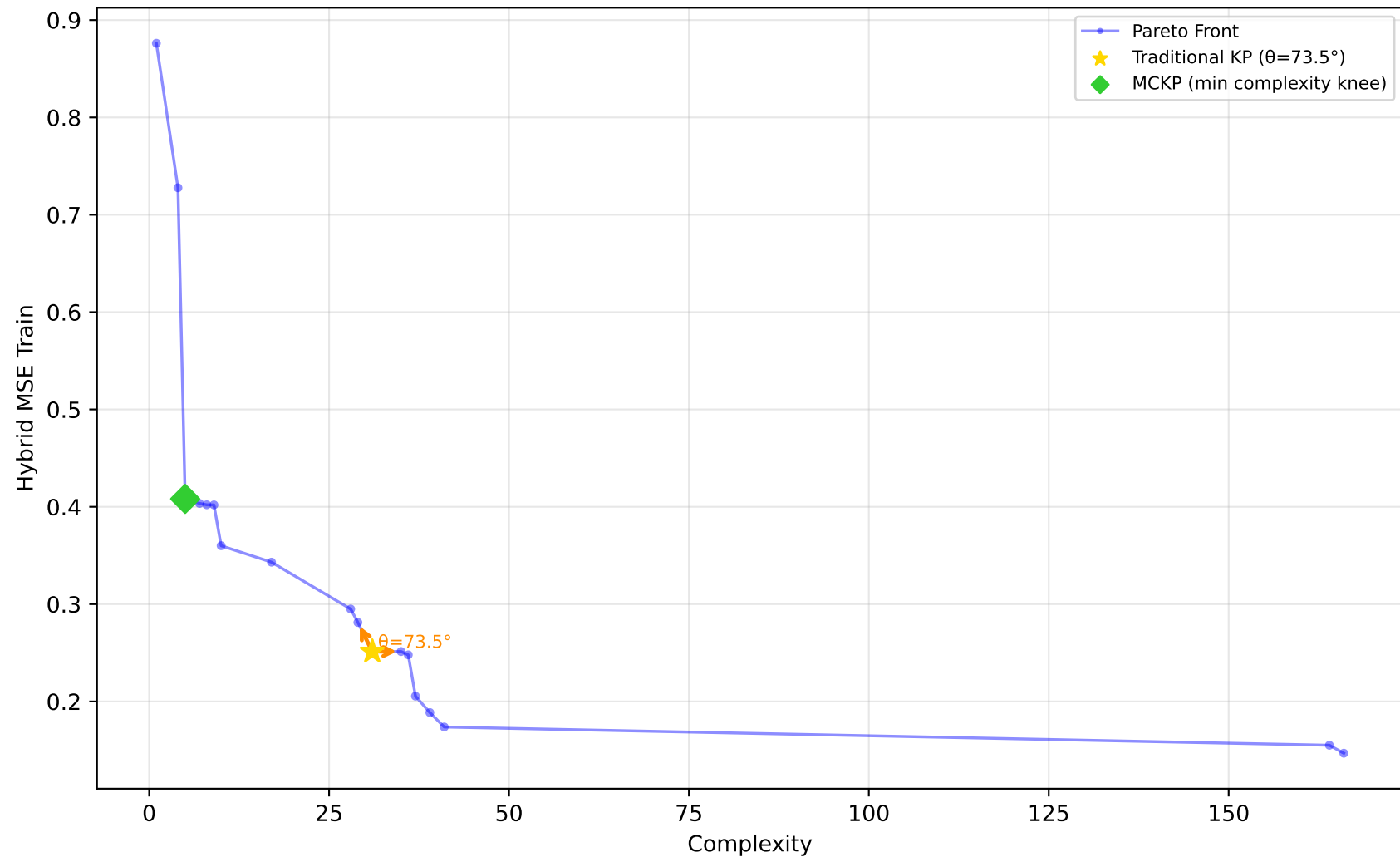
1028_SWD - Run 30 - MVP - Hybrid MSE Train \lambda_1=0.00, \lambda_2=0.00, \lambda_3=0.00 | Difficulty: 1.00 | Method: hmr
