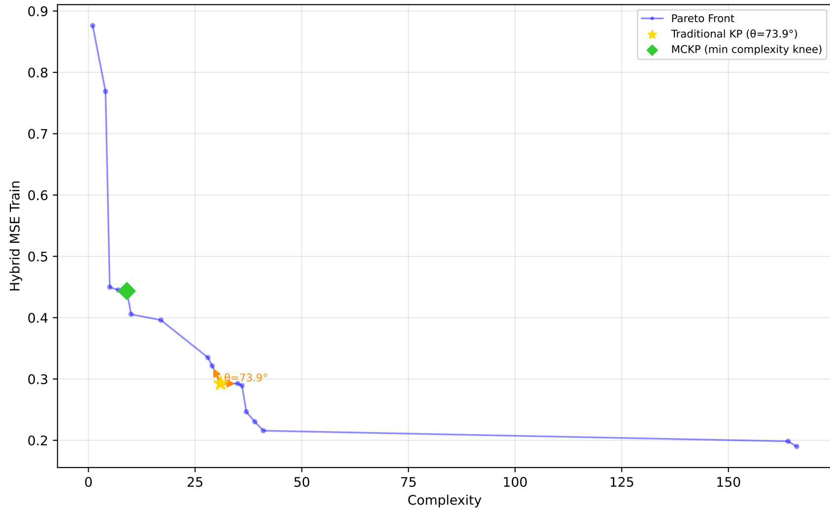
1028_SWD - Run 30 - MVP - Hybrid MSE Train \lambda_1=0.60, \lambda_2=0.00, \lambda_3=0.00 | Difficulty: 1.00 | Method: hmr
