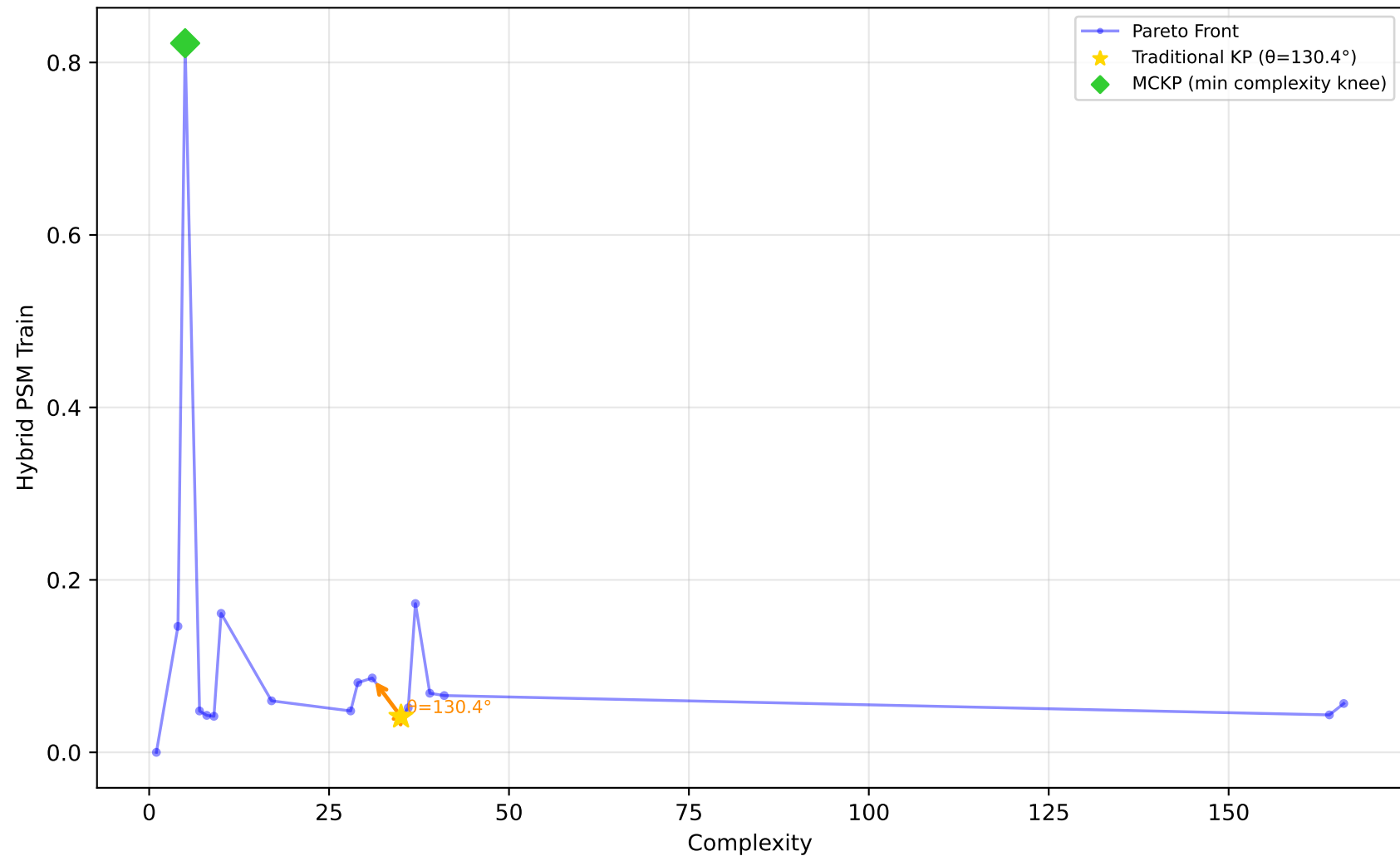
1028_SWD - Run 30 - MVP - Hybrid PSM Train \lambda_1=0.60, \lambda_2=0.00, \lambda_3=0.00 | Difficulty: 1.00 | Method: hmr
