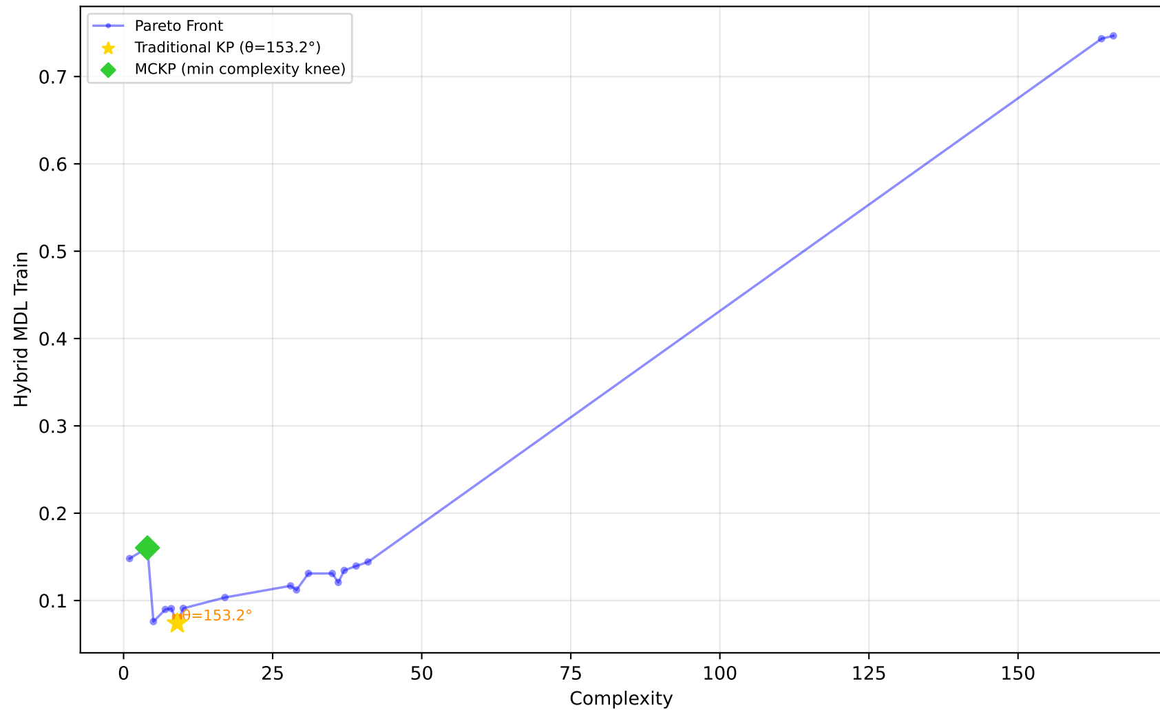
1028_SWD - Run 30 - SVP - Hybrid MDL Train \lambda_1=0.60, \lambda_2=0.00, \lambda_3=0.00 | Difficulty: 1.00 | Method: hmr
