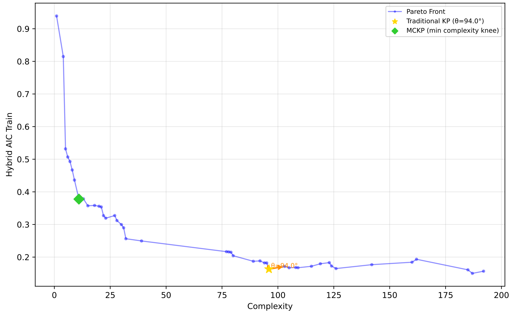
1028_SWD - Run 3 - MVP - Hybrid AIC Train \lambda_1=0.60, \lambda_2=0.00, \lambda_3=0.00 | Difficulty: 1.00 | Method: hmr
