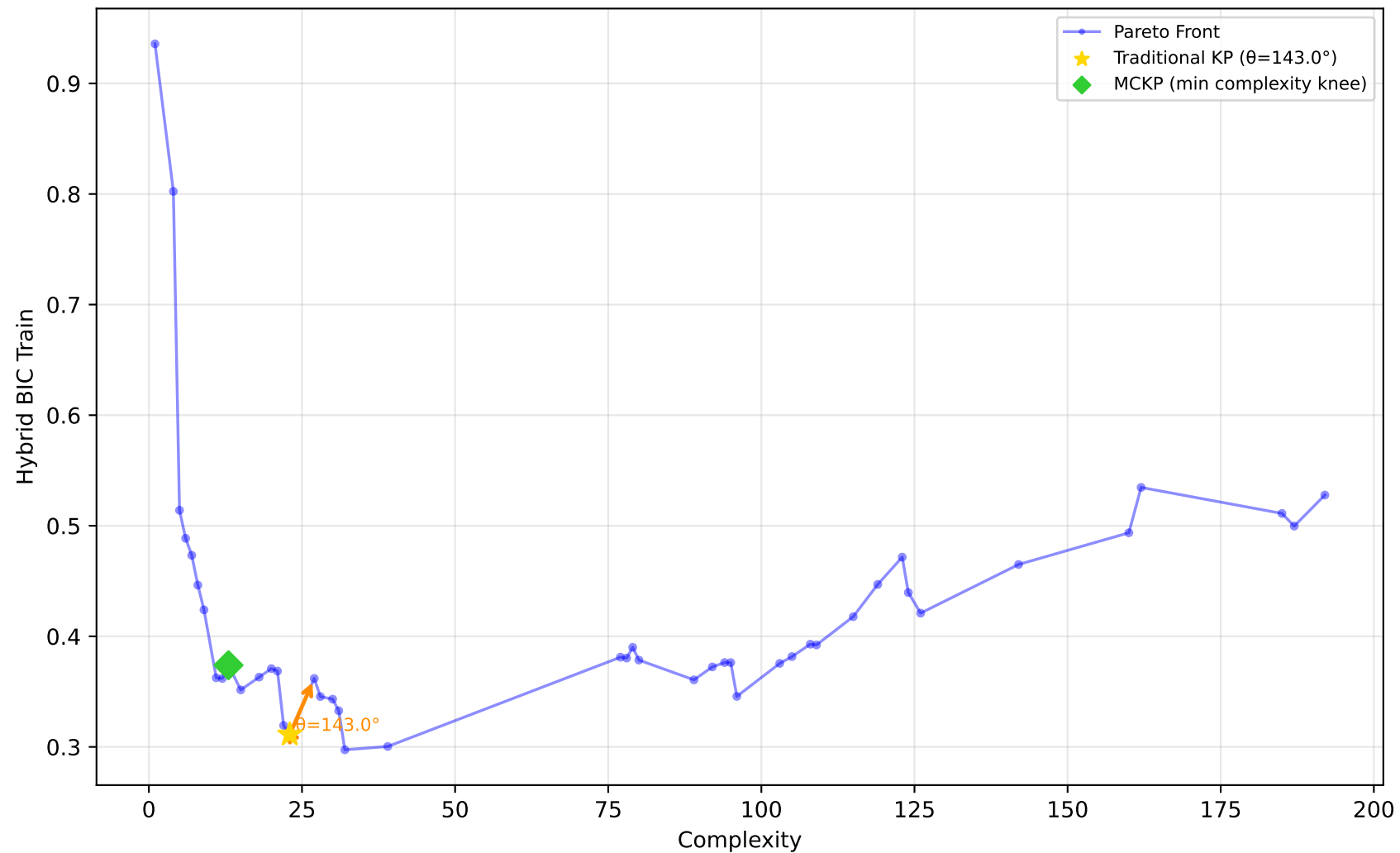
1028_SWD - Run 3 - MVP - Hybrid BIC Train \lambda_1=0.60, \lambda_2=0.00, \lambda_3=0.00 | Difficulty: 1.00 | Method: hmr
