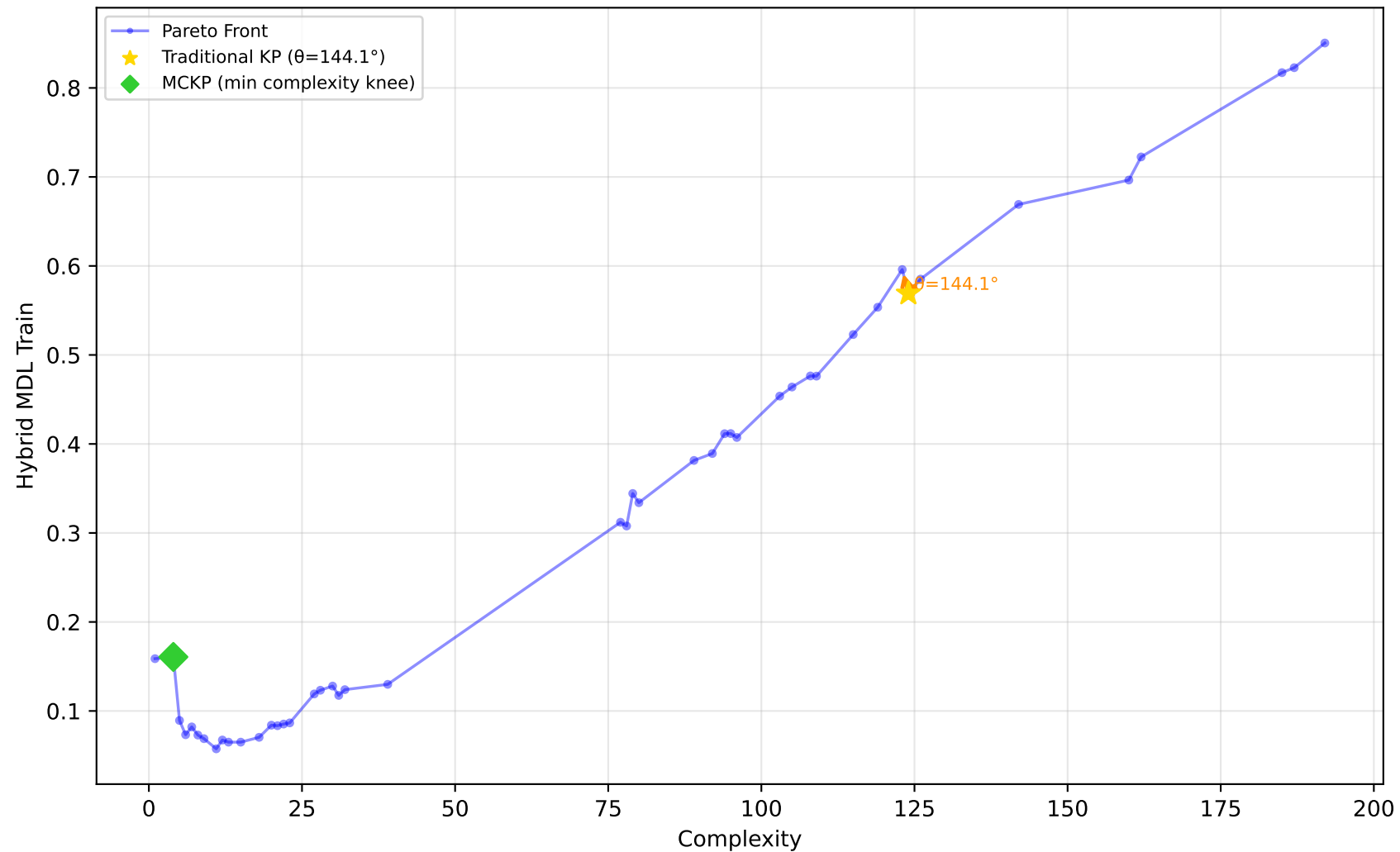
1028_SWD - Run 3 - MVP - Hybrid MDL Train \lambda_1=0.60, \lambda_2=0.00, \lambda_3=0.00 | Difficulty: 1.00 | Method: hmr
