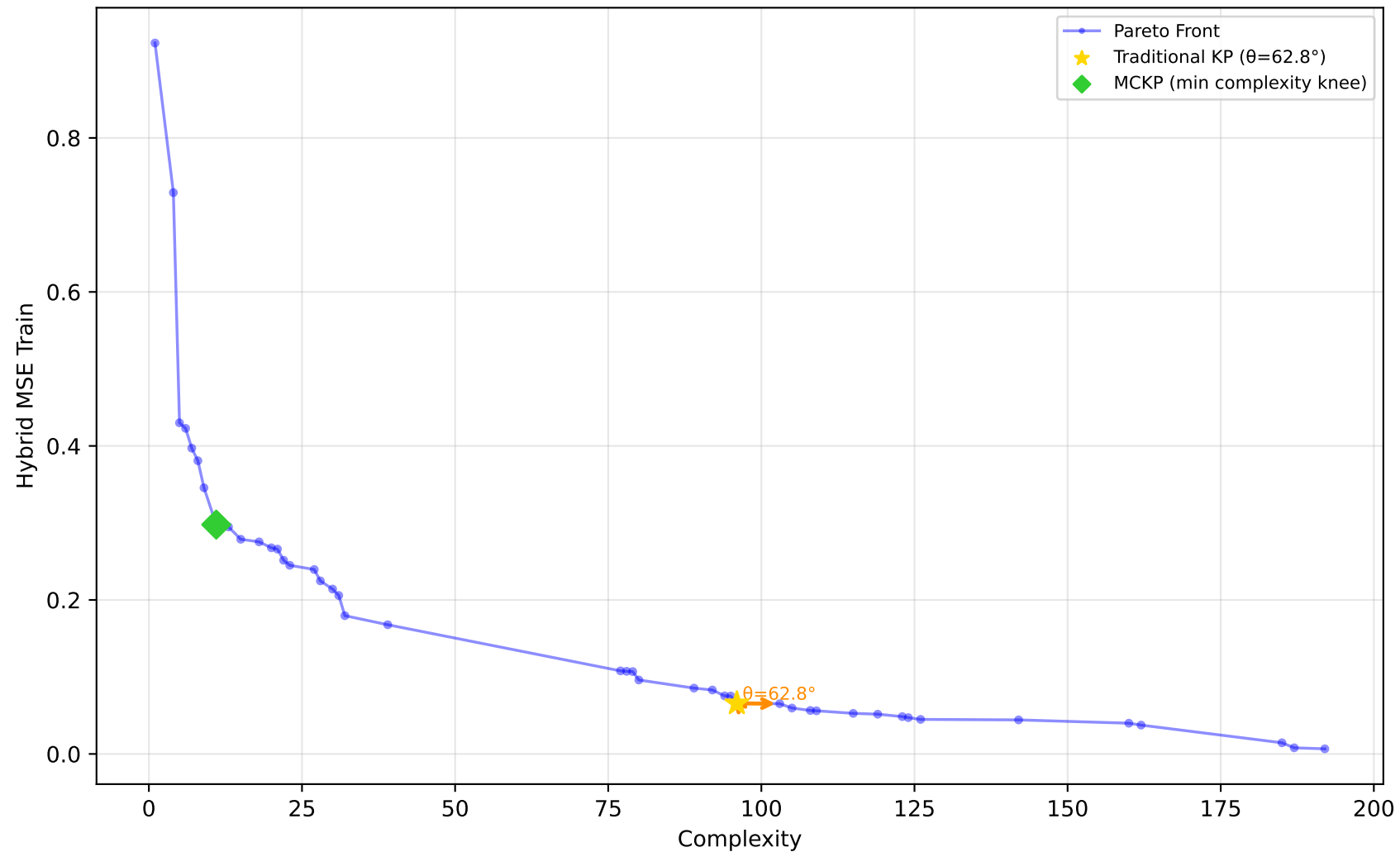
1028_SWD - Run 3 - MVP - Hybrid MSE Train \lambda_1=0.00, \lambda_2=0.00, \lambda_3=0.00 | Difficulty: 1.00 | Method: hmr
