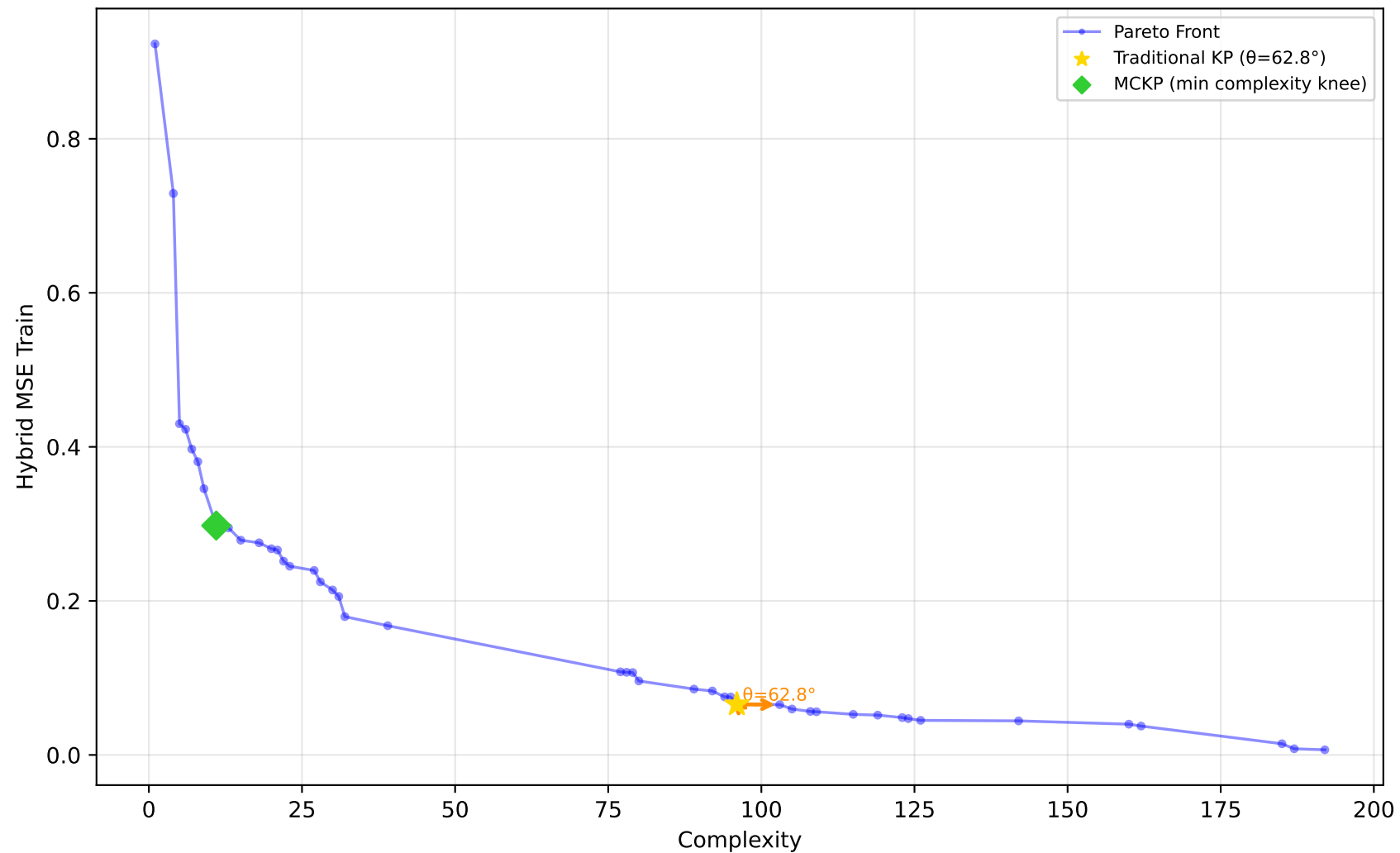
1028_SWD - Run 3 - SVP - Hybrid MSE Train \lambda_1=0.00, \lambda_2=0.60, \lambda_3=0.00 | Difficulty: 1.00 | Method: hmr
