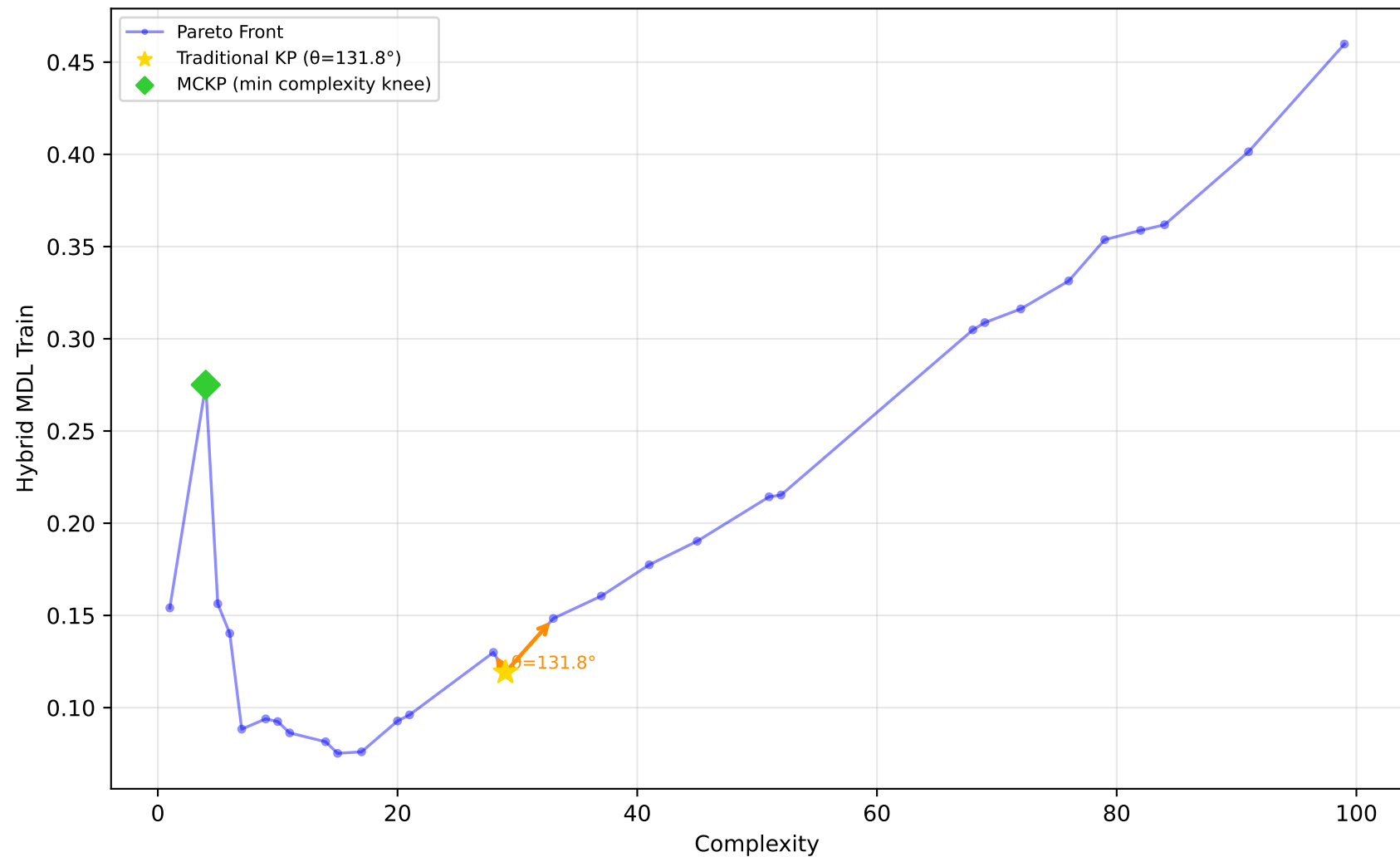
1028_SWD - Run 4 - MVP - Hybrid MDL Train \lambda_1=0.60, \lambda_2=0.00, \lambda_3=0.00 | Difficulty: 1.00 | Method: hmr
