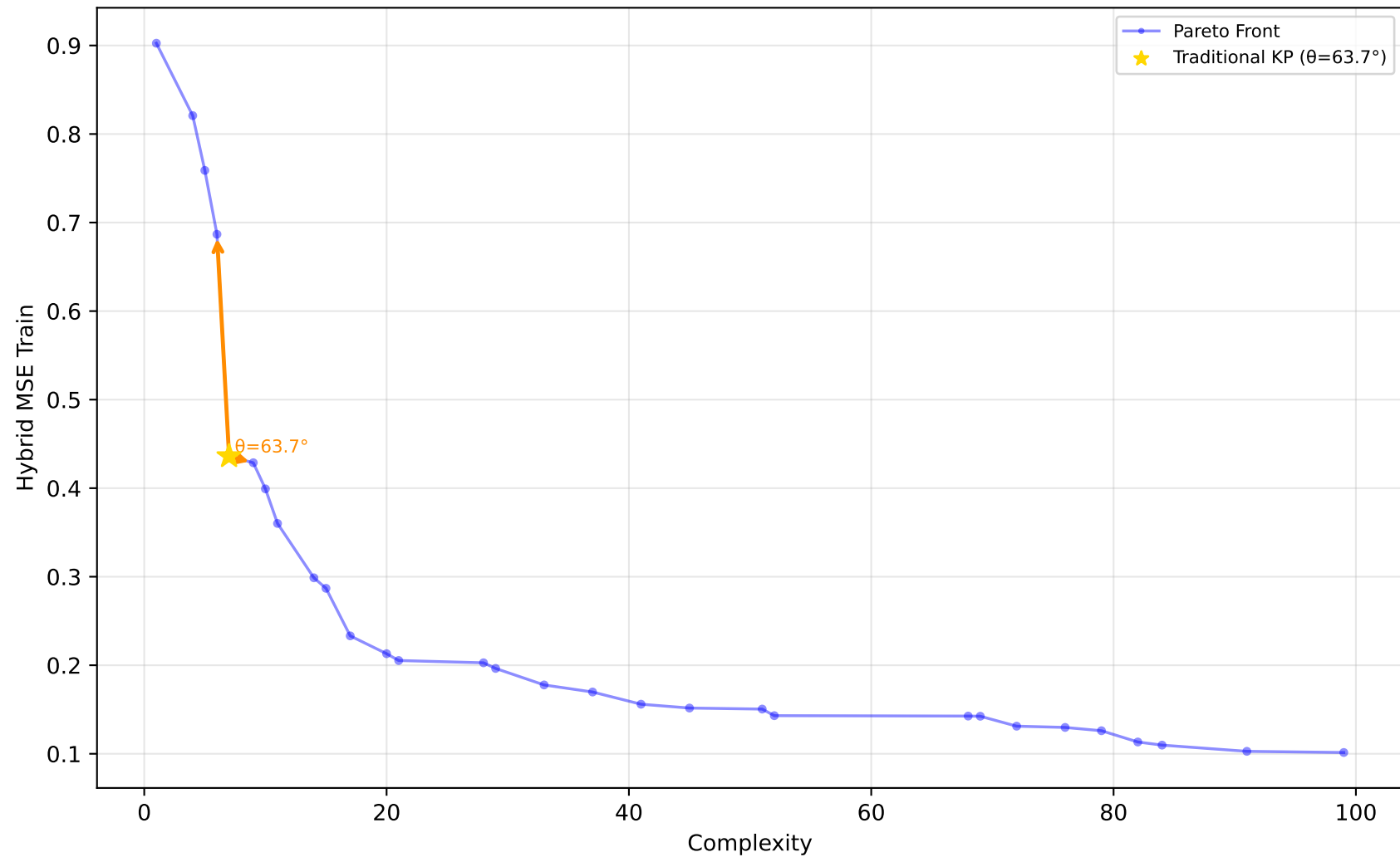
1028_SWD - Run 4 - MVP - Hybrid MSE Train \lambda_1=0.00, \lambda_2=0.00, \lambda_3=0.00 | Difficulty: 1.00 | Method: hmr
