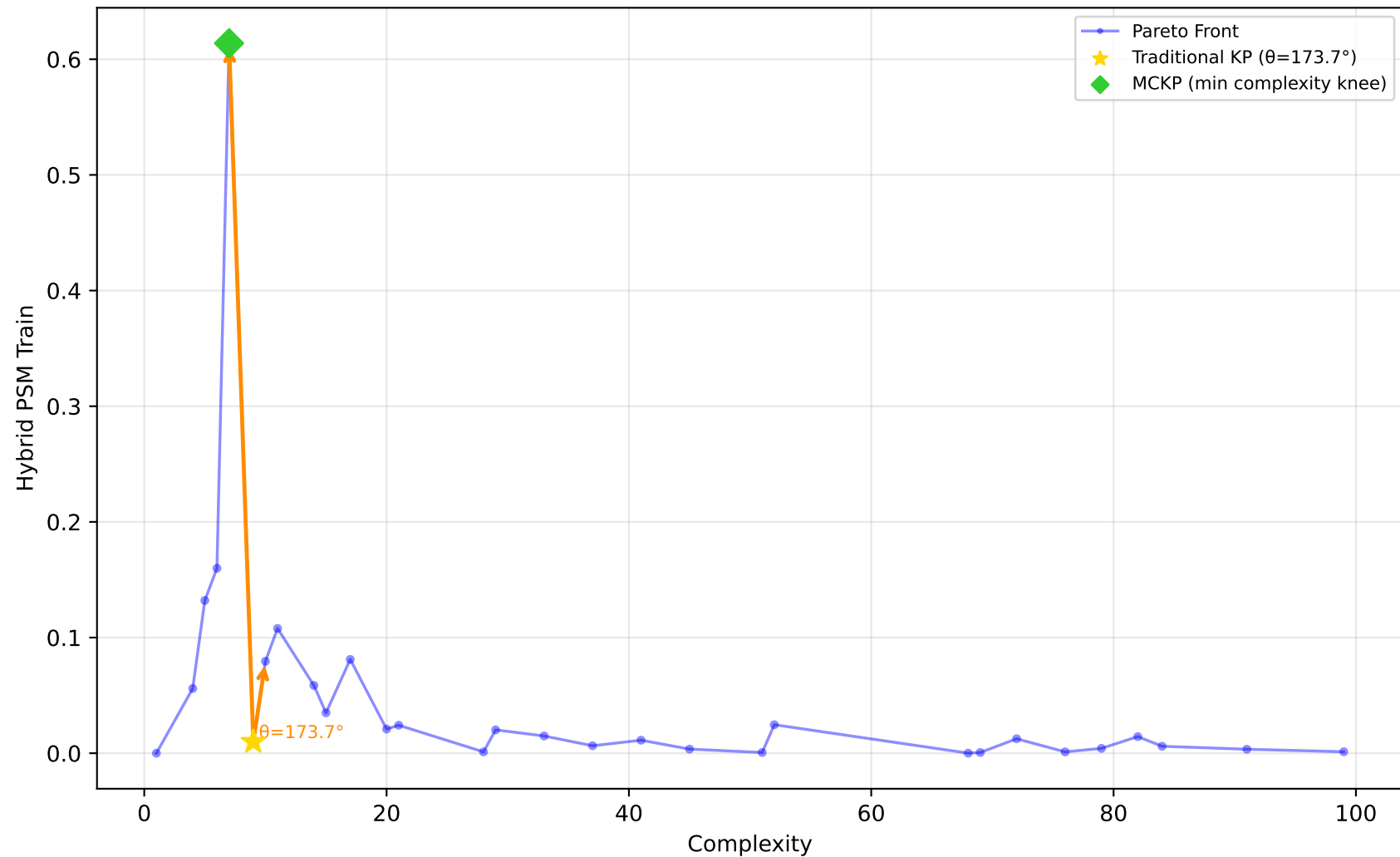
1028_SWD - Run 4 - MVP - Hybrid PSM Train \lambda_1=0.00, \lambda_2=0.00, \lambda_3=0.00 | Difficulty: 1.00 | Method: hmr
