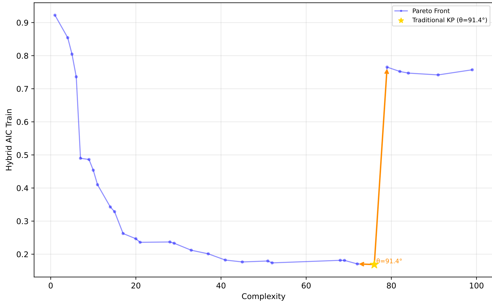
1028_SWD - Run 4 - SVP - Hybrid AIC Train \lambda_1=0.00, \lambda_2=0.60, \lambda_3=0.00 | Difficulty: 1.00 | Method: hmr
