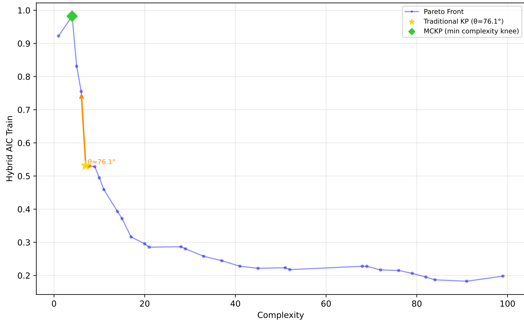
1028_SWD - Run 4 - SVP - Hybrid AIC Train \lambda_1=0.60, \lambda_2=0.00, \lambda_3=0.00 | Difficulty: 1.00 | Method: hmr
