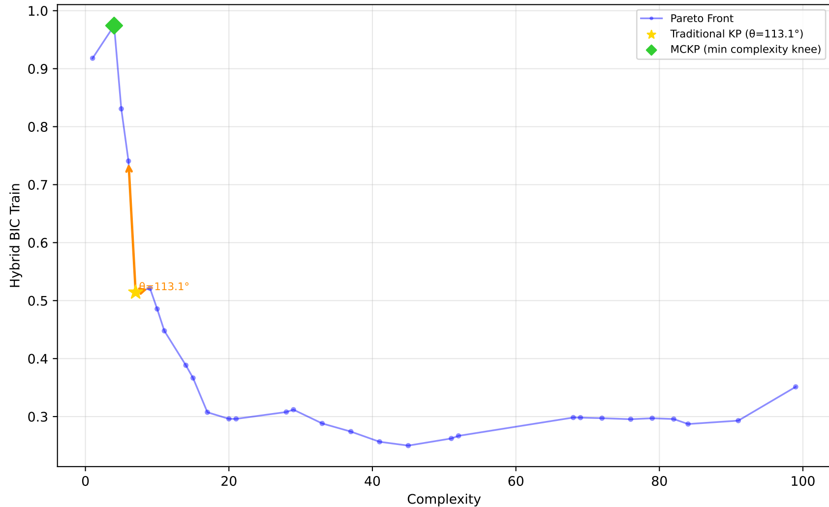
1028_SWD - Run 4 - SVP - Hybrid BIC Train \lambda_1=0.60, \lambda_2=0.00, \lambda_3=0.00 | Difficulty: 1.00 | Method: hmr
