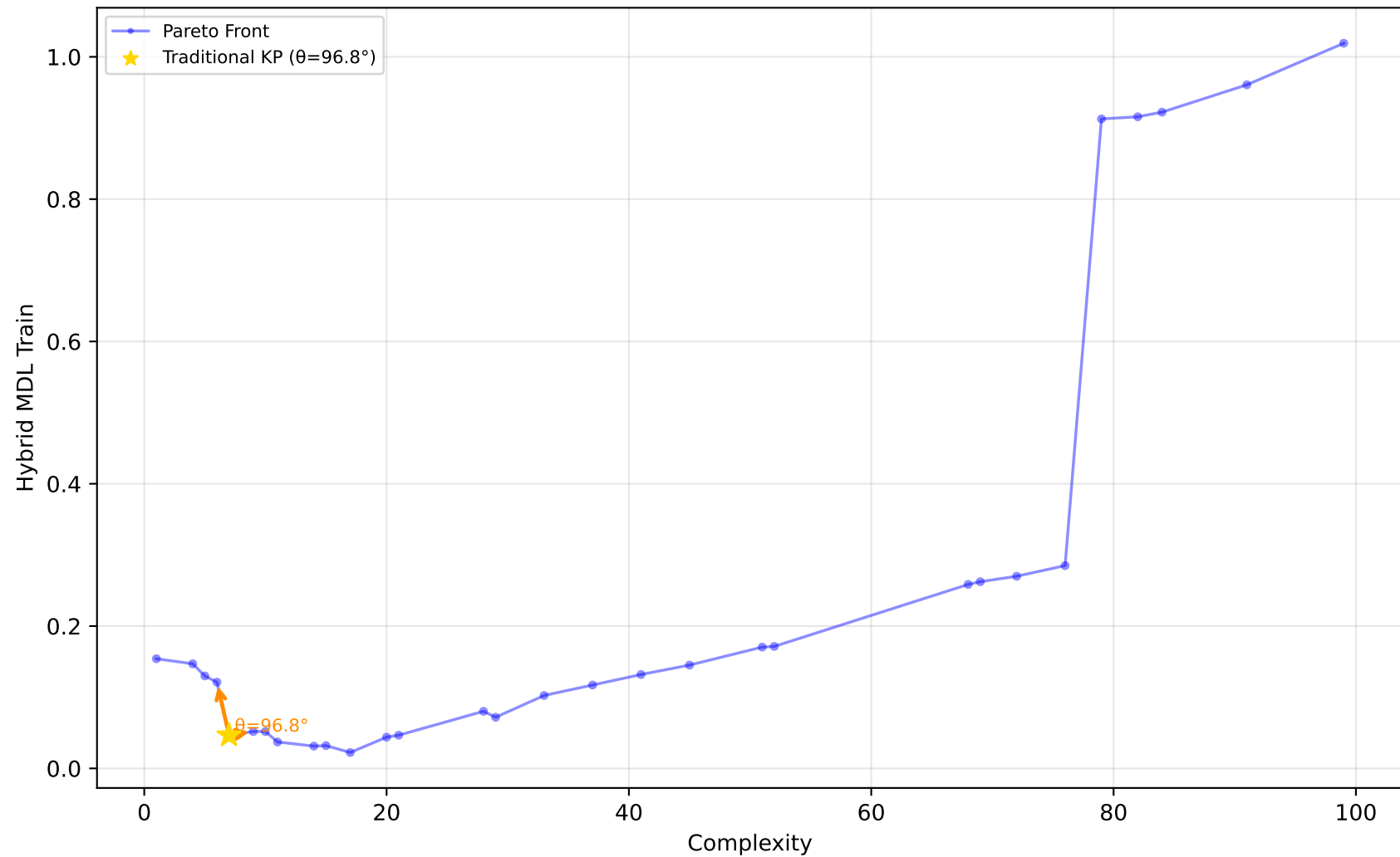
1028_SWD - Run 4 - SVP - Hybrid MDL Train \lambda_1=0.00, \lambda_2=0.60, \lambda_3=0.00 | Difficulty: 1.00 | Method: hmr
