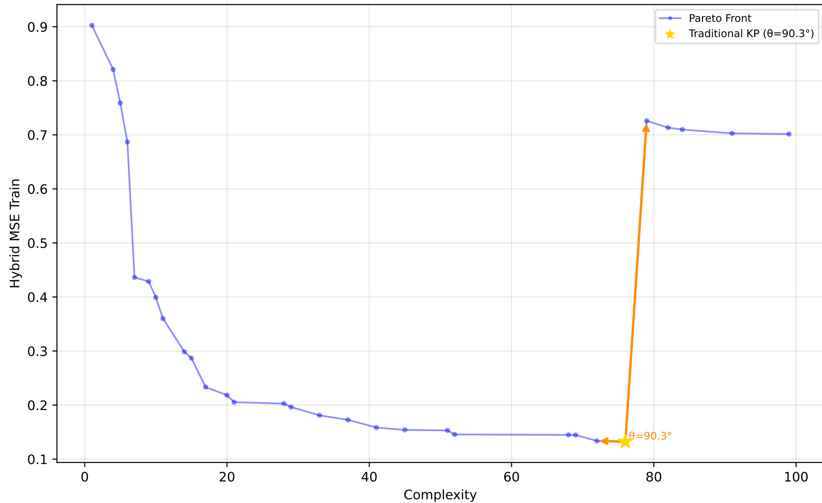
1028_SWD - Run 4 - SVP - Hybrid MSE Train \lambda_1=0.00, \lambda_2=0.60, \lambda_3=0.00 | Difficulty: 1.00 | Method: hmr
