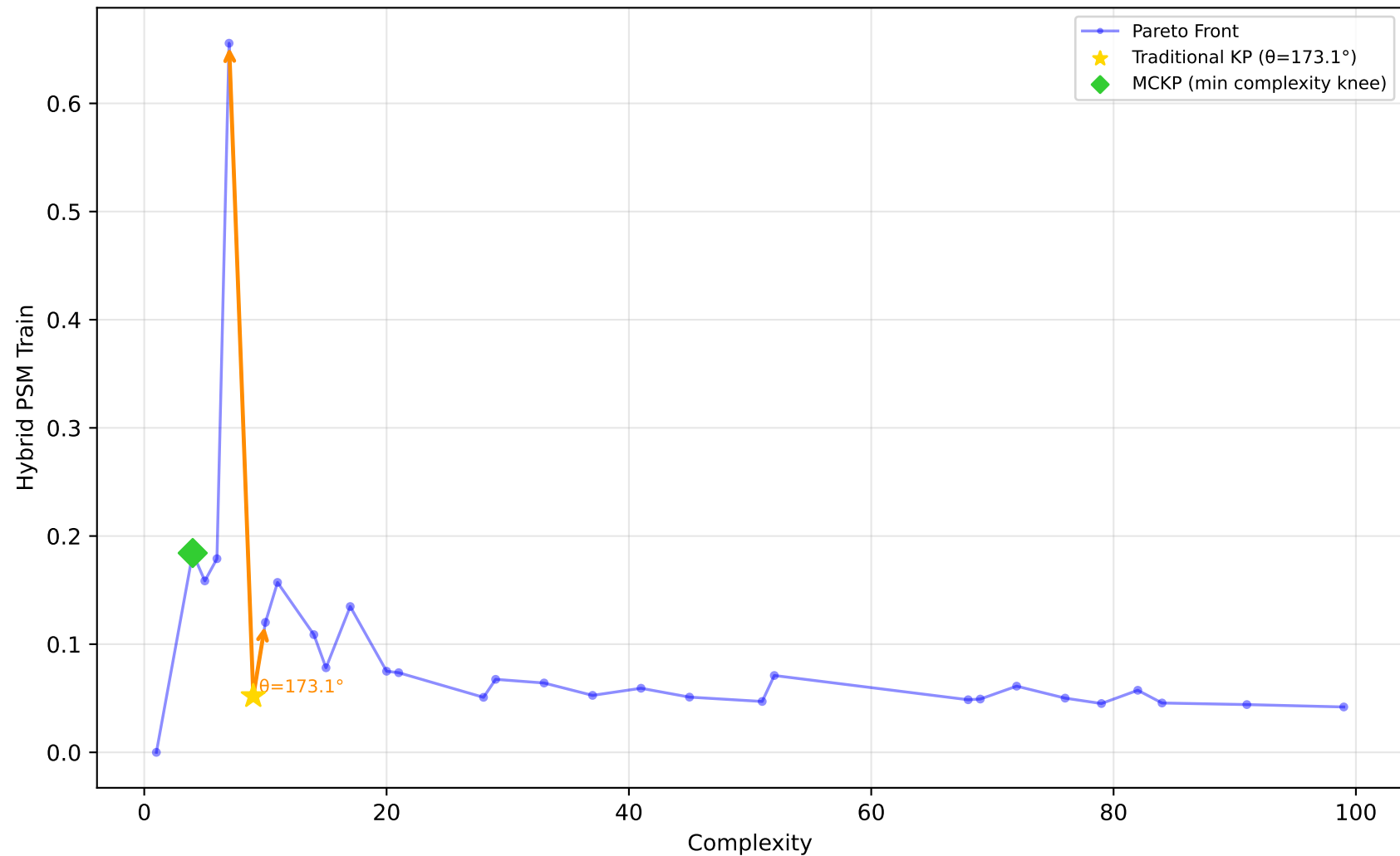
1028_SWD - Run 4 - SVP - Hybrid PSM Train \lambda_1=0.60, \lambda_2=0.00, \lambda_3=0.00 | Difficulty: 1.00 | Method: hmr
