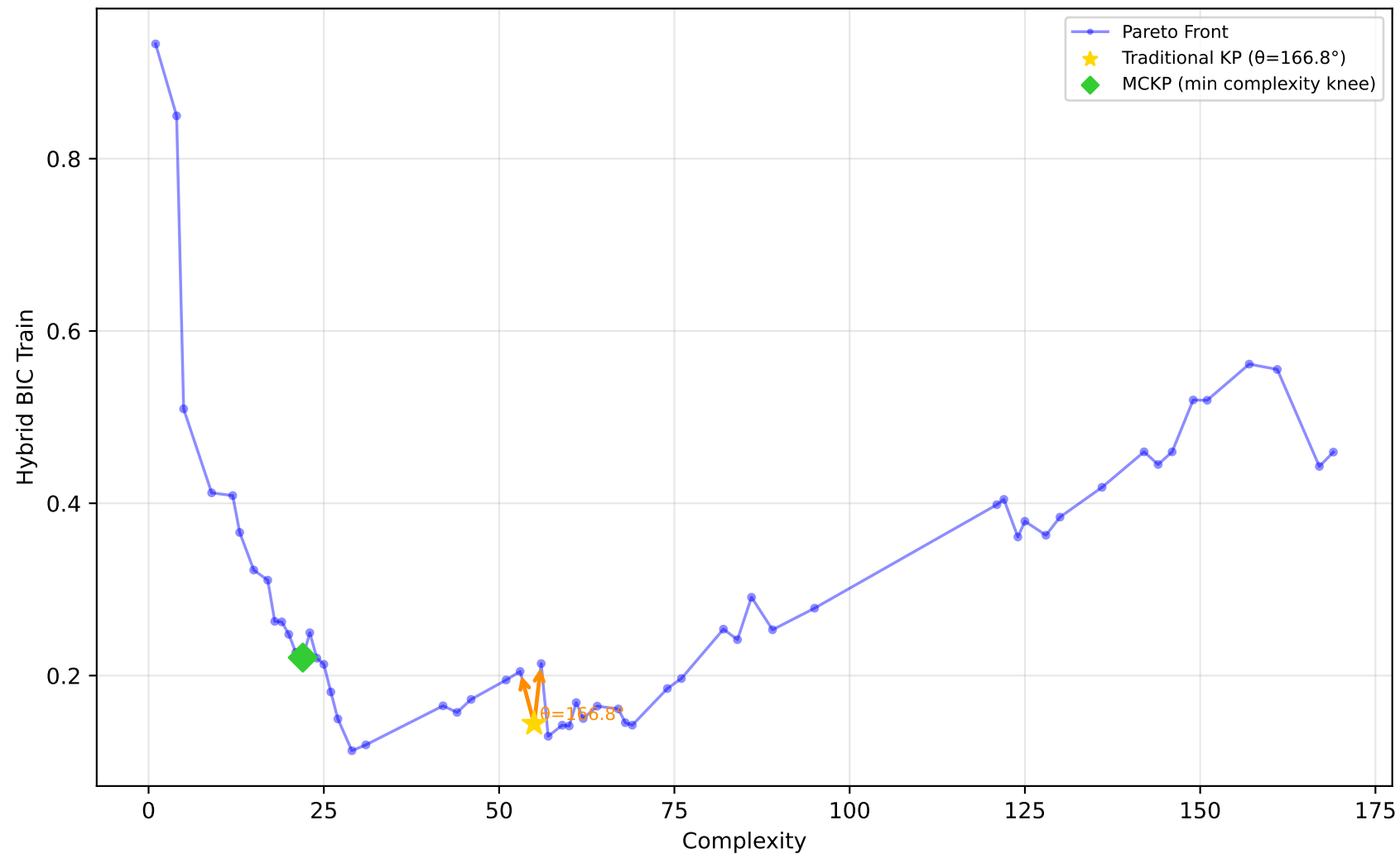
1028_SWD - Run 5 - MVP - Hybrid BIC Train \lambda_1=0.60, \lambda_2=0.00, \lambda_3=0.00 | Difficulty: 0.79 | Method: hmr
