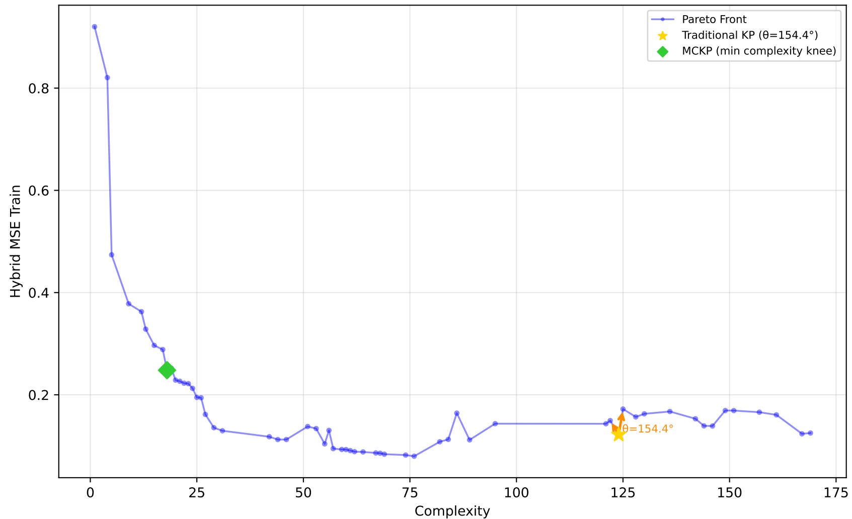
1028_SWD - Run 5 - MVP - Hybrid MSE Train \lambda_1=0.60, \lambda_2=0.00, \lambda_3=0.00 | Difficulty: 0.79 | Method: hmr
