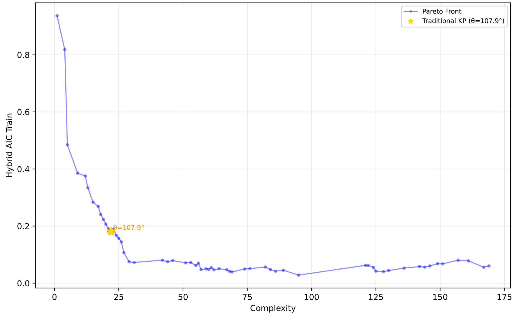
1028_SWD - Run 5 - SVP - Hybrid AIC Train \lambda_1=0.00 , \lambda_2=0.60 , \lambda_3=0.00 | Difficulty: 0.79 | Method: hmr
