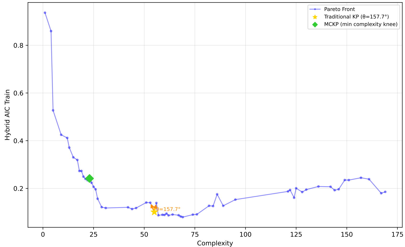
1028_SWD - Run 5 - SVP - Hybrid AIC Train \lambda_1=0.60, \lambda_2=0.00, \lambda_3=0.00 | Difficulty: 0.79 | Method: hmr
