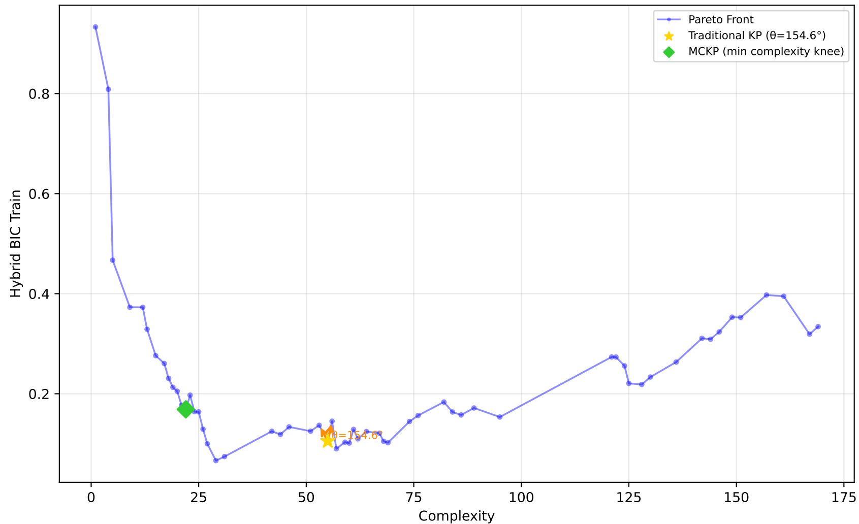
1028_SWD - Run 5 - SVP - Hybrid BIC Train \lambda_1=0.00 , \lambda_2=0.60 , \lambda_3=0.00 | Difficulty: 0.79 | Method: hmr
