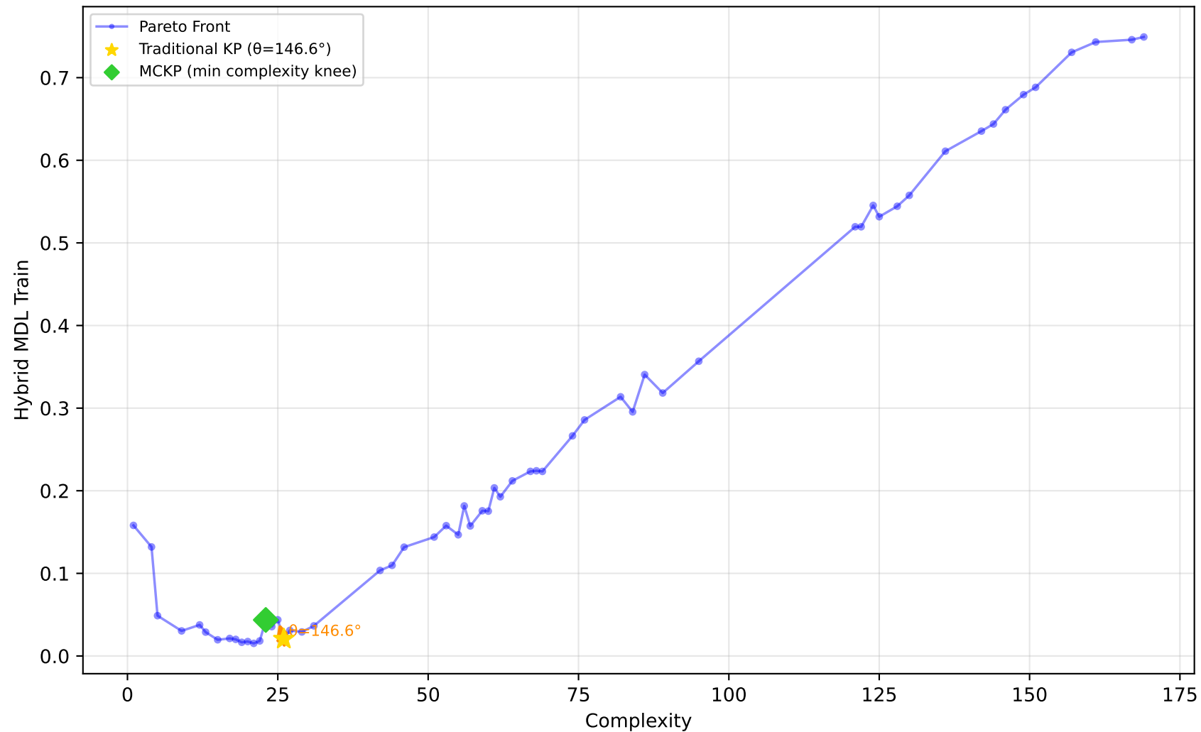
1028_SWD - Run 5 - SVP - Hybrid MDL Train \lambda_1=0.00, \lambda_2=0.60, \lambda_3=0.00 | Difficulty: 0.79 | Method: hmr
