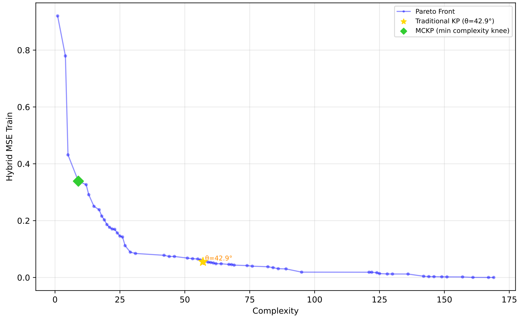
1028_SWD - Run 5 - SVP - Hybrid MSE Train \lambda_1=0.00, \lambda_2=0.60, \lambda_3=0.00 | Difficulty: 0.79 | Method: hmr
