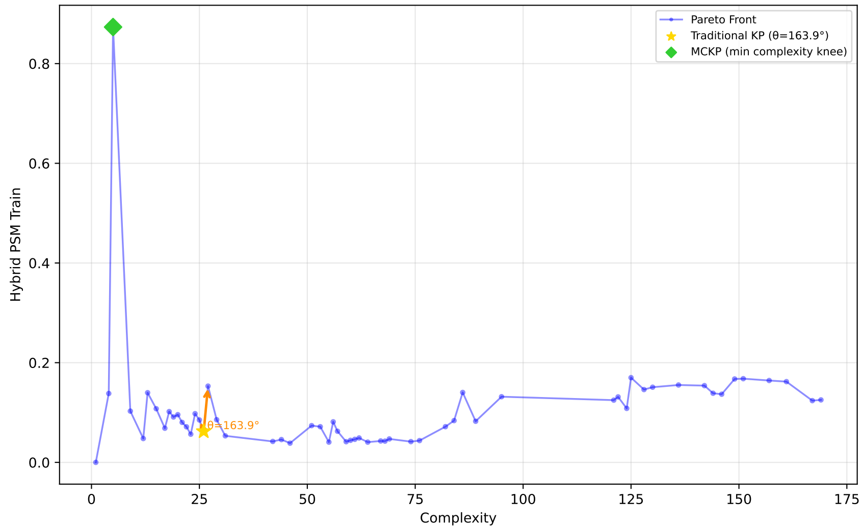
1028_SWD - Run 5 - SVP - Hybrid PSM Train \lambda_1=0.60, \lambda_2=0.00, \lambda_3=0.00 | Difficulty: 0.79 | Method: hmr
