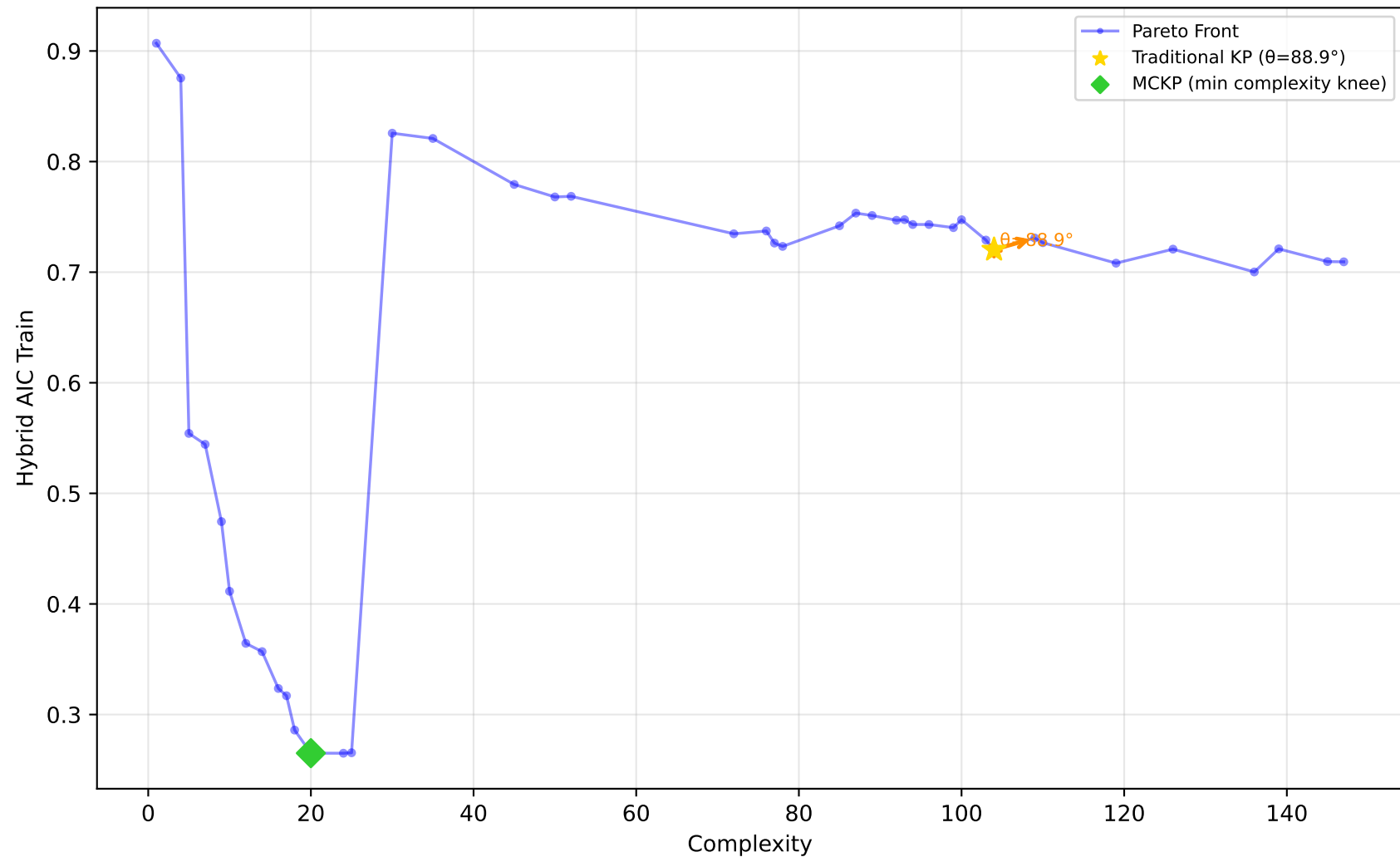
1028_SWD - Run 6 - MVP - Hybrid AIC Train \lambda_1=0.60, \lambda_2=0.00, \lambda_3=0.00 | Difficulty: 1.00 | Method: hmr
