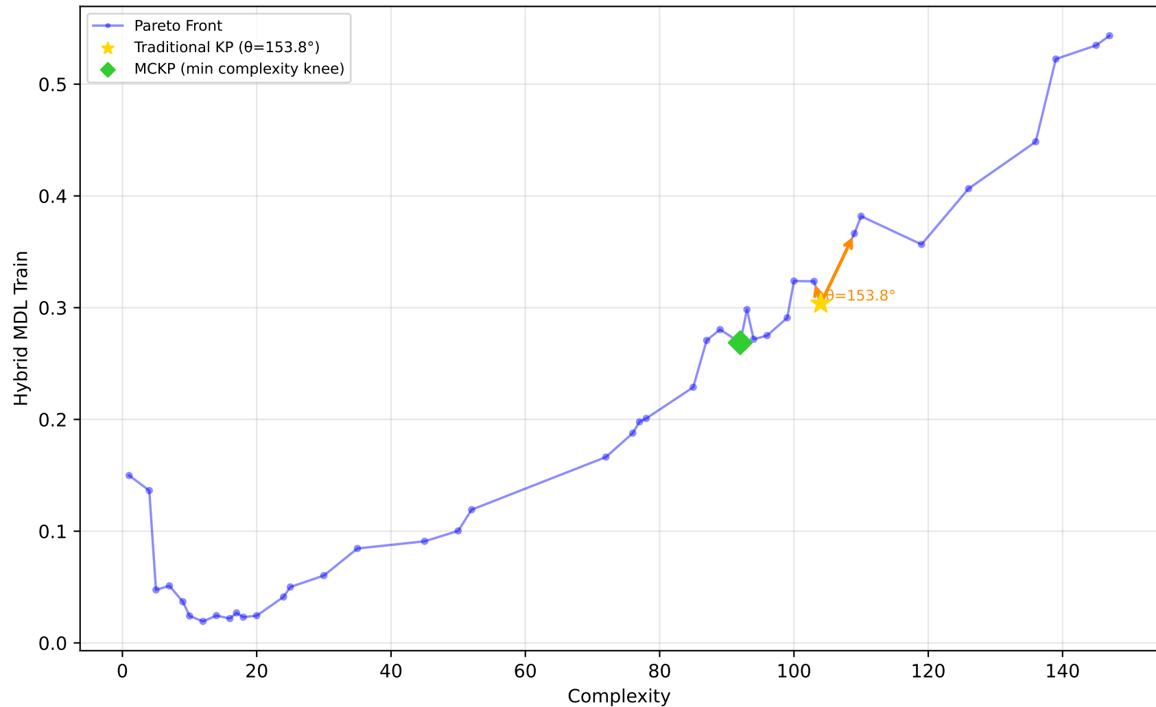
1028_SWD - Run 6 - MVP - Hybrid MDL Train \lambda_1=0.00, \lambda_2=0.00, \lambda_3=0.00 | Difficulty: 1.00 | Method: hmr
