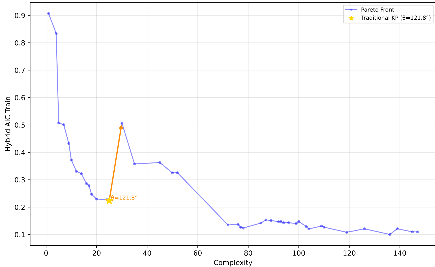
1028_SWD - Run 6 - SVP - Hybrid AIC Train \lambda_1=0.00, \lambda_2=0.60, \lambda_3=0.00 | Difficulty: 1.00 | Method: hmr
