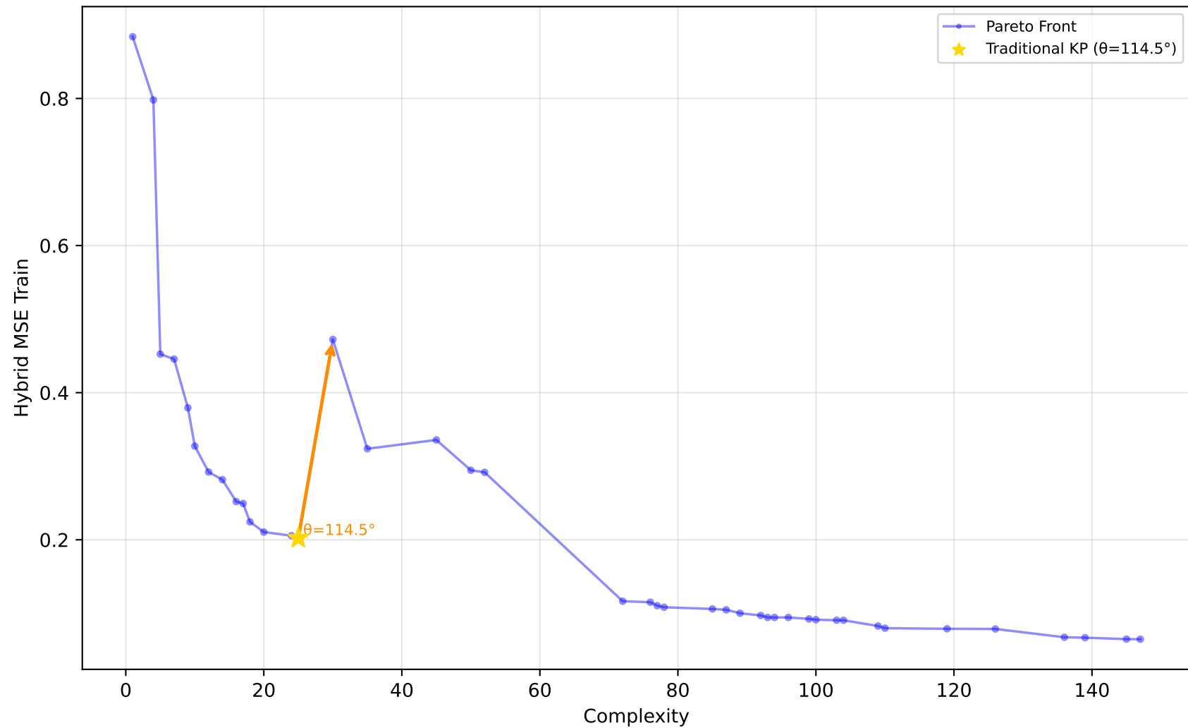
1028_SWD - Run 6 - SVP - Hybrid MSE Train \lambda_1=0.00, \lambda_2=0.60, \lambda_3=0.00 | Difficulty: 1.00 | Method: hmr
