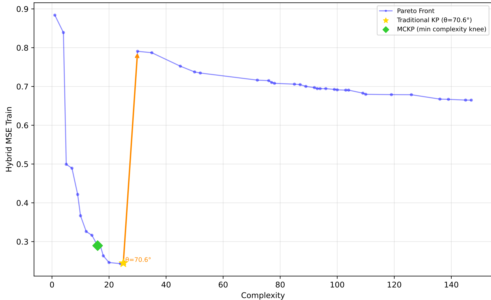
1028_SWD - Run 6 - SVP - Hybrid MSE Train \lambda_1=0.60, \lambda_2=0.00, \lambda_3=0.00 | Difficulty: 1.00 | Method: hmr
