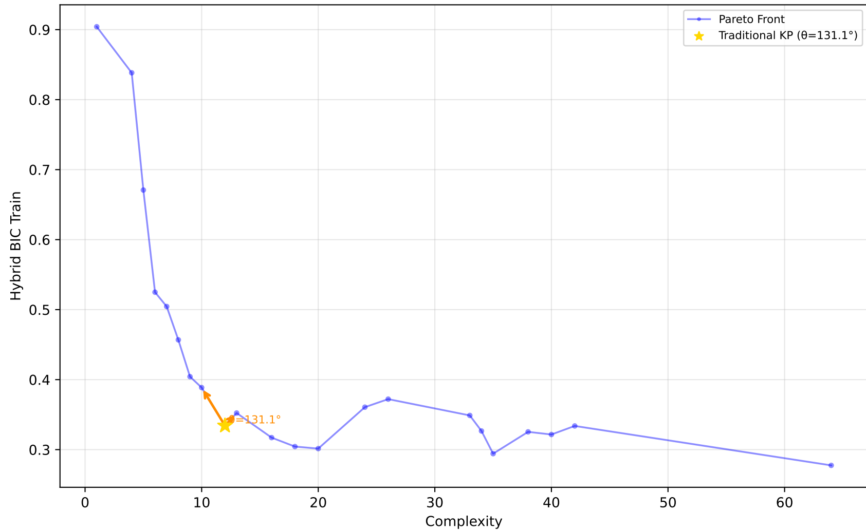
1028_SWD - Run 7 - MVP - Hybrid BIC Train \lambda_1=0.00, \lambda_2=0.00, \lambda_3=0.00 | Difficulty: 1.00 | Method: hmr
