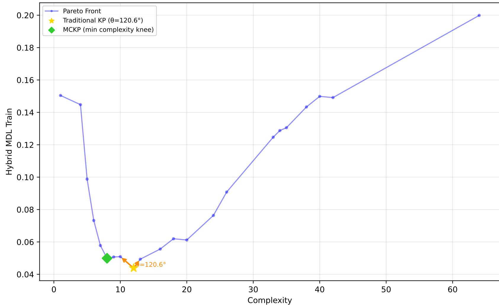
1028_SWD - Run 7 - MVP - Hybrid MDL Train \lambda_1=0.00, \lambda_2=0.00, \lambda_3=0.00 | Difficulty: 1.00 | Method: hmr
