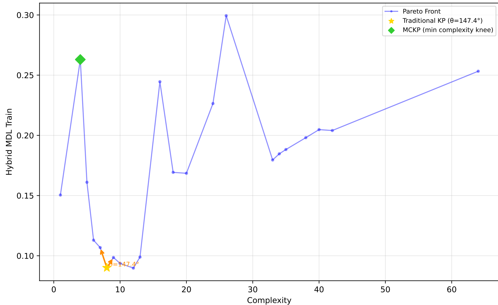
1028_SWD - Run 7 - MVP - Hybrid MDL Train \lambda_1=0.60, \lambda_2=0.00, \lambda_3=0.00 | Difficulty: 1.00 | Method: hmr
