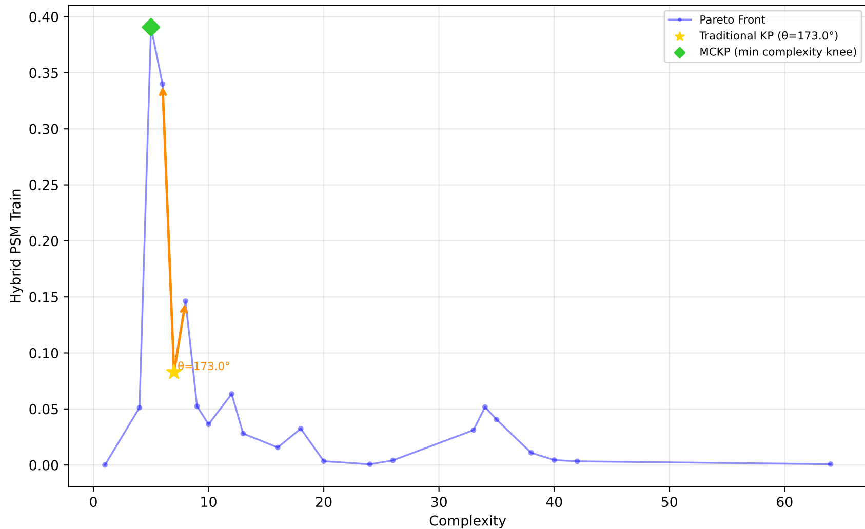
1028_SWD - Run 7 - MVP - Hybrid PSM Train \lambda_1=0.00, \lambda_2=0.00, \lambda_3=0.00 | Difficulty: 1.00 | Method: hmr
