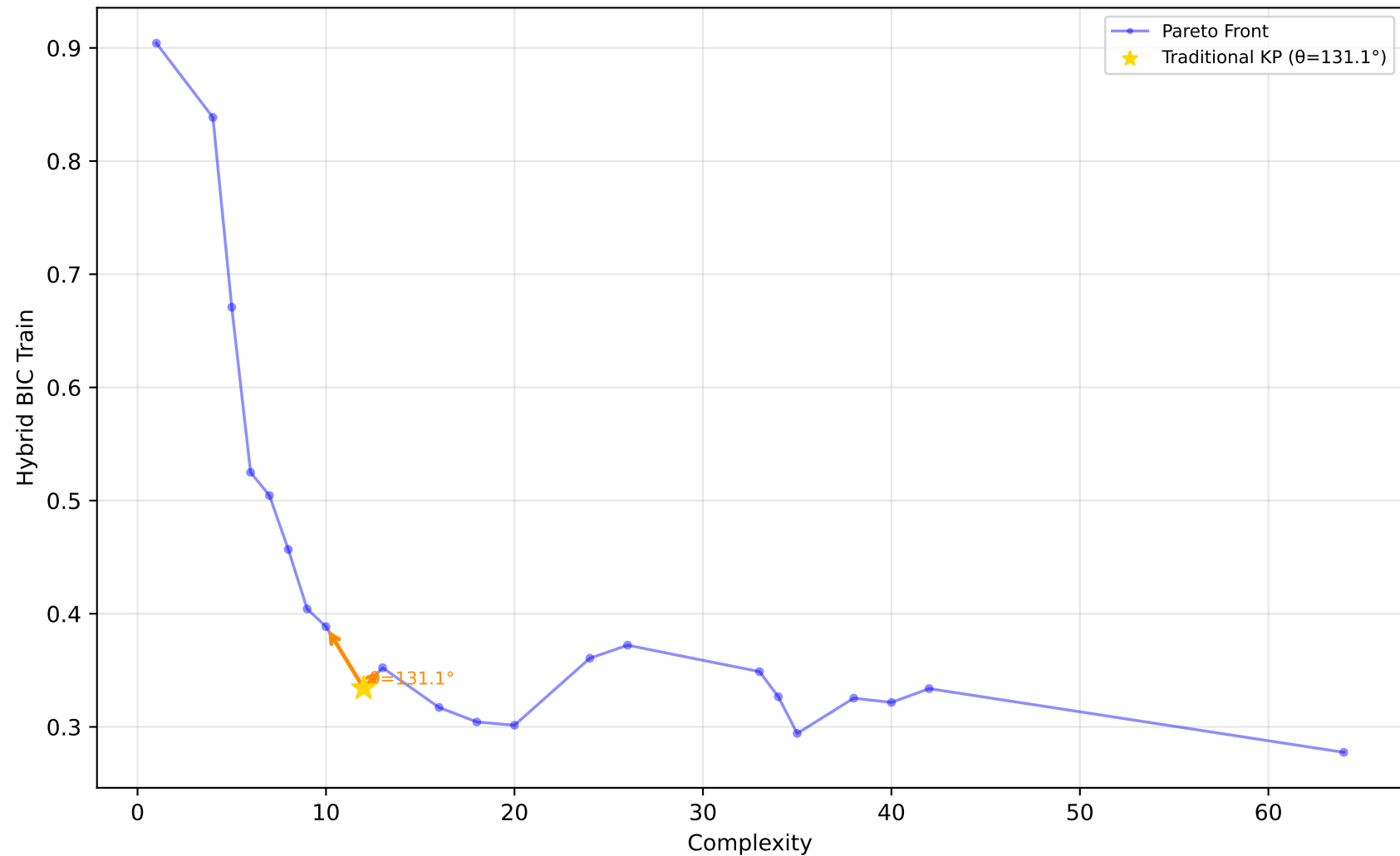
1028_SWD - Run 7 - SVP - Hybrid BIC Train \lambda_1=0.00, \lambda_2=0.60, \lambda_3=0.00 | Difficulty: 1.00 | Method: hmr
