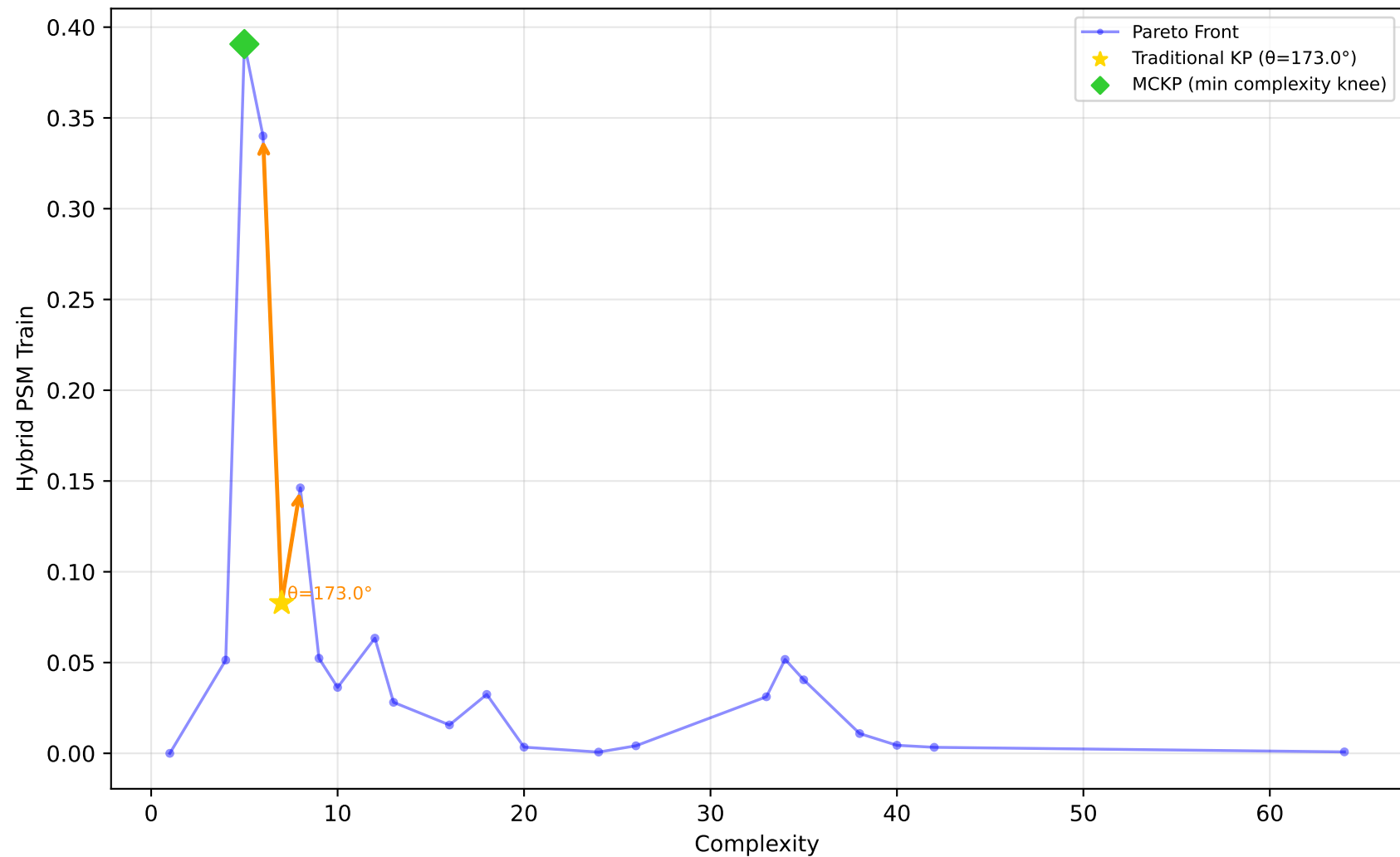
1028_SWD - Run 7 - SVP - Hybrid PSM Train \lambda_1=0.00 , \lambda_2=0.60 , \lambda_3=0.00 | Difficulty: 1.00 | Method: hmr
