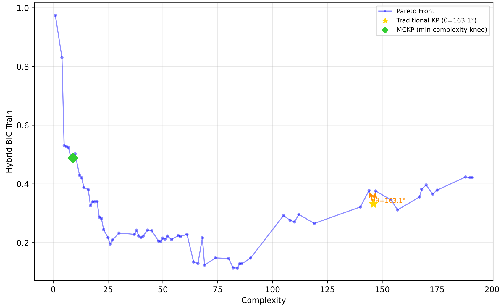
1028_SWD - Run 8 - MVP - Hybrid BIC Train \lambda_1=0.00, \lambda_2=0.00, \lambda_3=0.00 | Difficulty: 1.00 | Method: hmr
